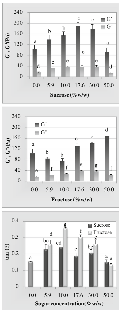
Fig. 3 The elastic ( G' ) and viscous ( G'' ) moduli at different sugar concentrations for sucrose (a) or fructose (b) and the loss tangent ( \tan \delta ) at the same concentrations of both sugars (c)—all at a frequency of 1 Hz and 20 °C. Within the same graph and in the same parameter different letters above the error bars indicate significant differences ( p \leq 0.05 )
