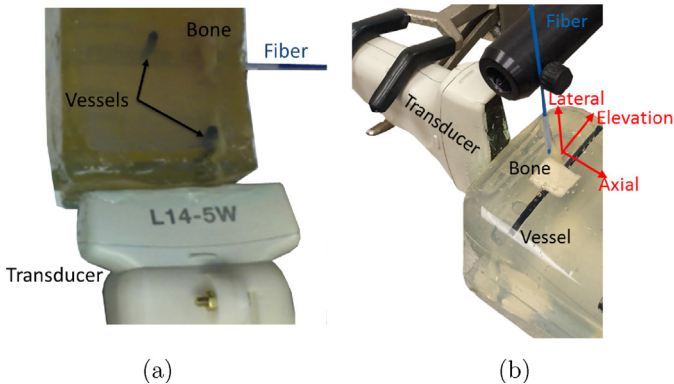
Fig. 2. Photoacoustic experimental setup for (a) bone visualization and (b) fiber translation.
