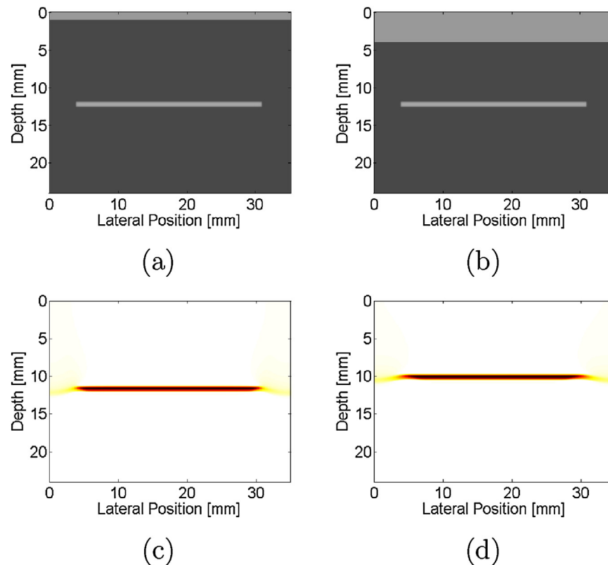
Fig. 3. Simulated phantom with (a) 1-mm and (b) 4-mm thick temporal bone located at the sensor surface (depth = 0 mm) and horizontal target located at a depth of 12 mm. Corresponding simulated photoacoustic images, demonstrating that as the temporal bone thickness increases from (c) 1 mm to (d) 4 mm, the target appears closer to the ultrasound sensor.
