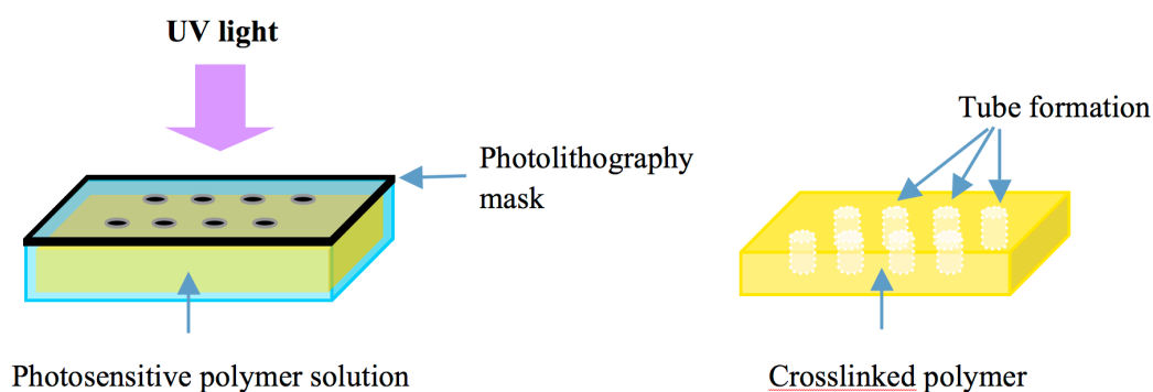
Figure 4. Photopatterning approach for fabrication of microfluidic constructs. A thin film of a photosensitive polymer is exposed to UV light through a predefined mask. There are transparent regions in the mask that allow the UV light to pass through. The areas where the light can reach through the transparent regions generate crosslinking of the polymer while the dark areas under the mask that cannot receive the light will maintain liquid and can be easily removed to form tubular structures.
