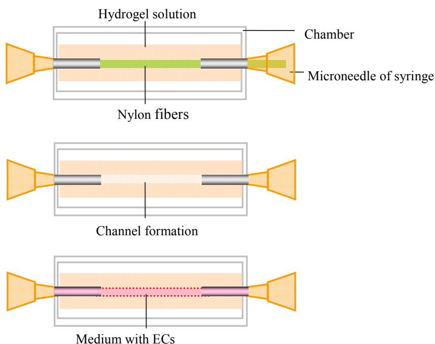
Figure 2. Molding approach for fabrication of microfluidic constructs. Microneedles and a Nylon fiber are fixed inside a chamber. Then hydrogel solutions are poured into the chamber and gelled. Then open channels are formed by gently removing the fibers. Medium with ECs can be perfused through the channel.
