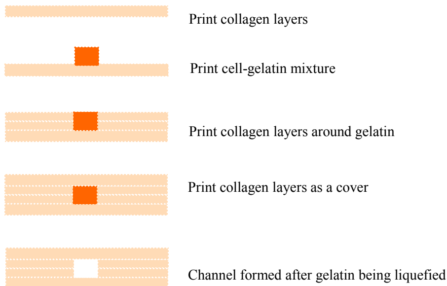
Figure 5. Bioprinting for fabrication of multi-level tubular constructs. With a layer-by-layer printing approach, the collagen precursor was printed and polymerized. Then gelatin/cell mixture was printed in a straight pattern to take the position of the channel. After gelation, more collagen layers were printed to cover the gelatin pattern. The vascular structure was formed after gelatin was liquefied.
