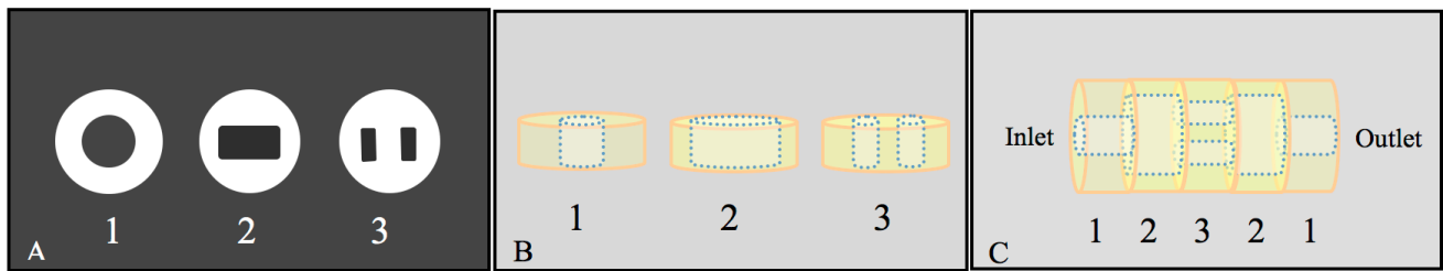
Figure 6. Modular method for fabricating multi-level tubular constructs. (A) The Mask with multi-level tubular structure for a photopatterning approach; (B) The microtubes created after UV-light photocuring; (C) Microtubes are assembled into a larger and longer tubular construct with multi-level interconnected lumens.
