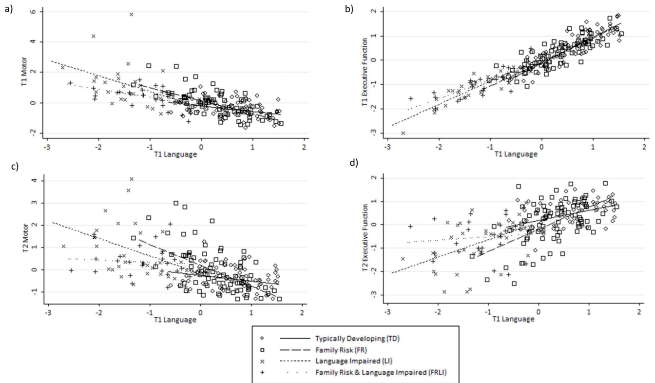
Figure 3. Scatter plots illustrating the relationships between T1 Language and T1 Motor (a), T1 Executive Function (b), T2 Motor (c) and T2 Executive Function (d) factor scores.
