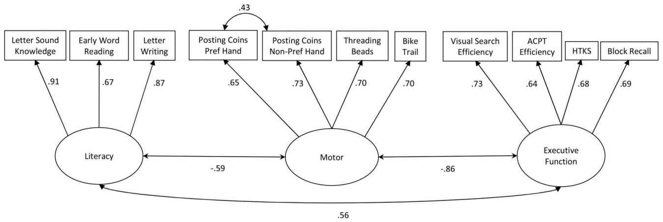
Figure 2. Confirmatory Factor Analysis of T2 literacy, motor and executive function variables. \chi^2(40) = 70.881, p = 0.002 ; RMSEA = 0.060; CFI = 0.969; TLI = 0.957
