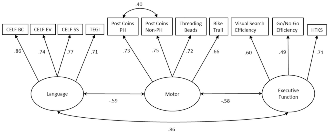
Figure 1. Confirmatory factor analysis of the T1 language, motor and executive function variables. \chi^2(40) = 59.891, p = 0.022 ; RMSEA = 0.048; CFI = 0.974; TLI = 0.964
