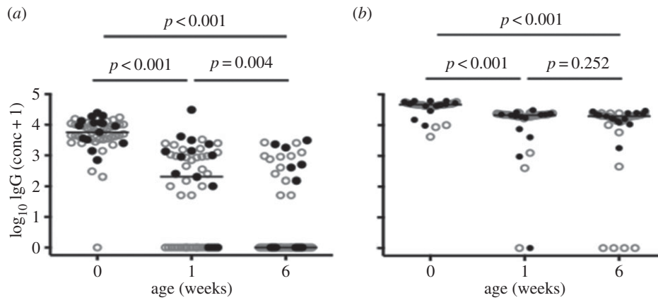
Figure 2. Longitudinal changes in \log_{10} (concentration+1) PPD- (a) and TT-specific (b) IgG concentrations. Cord blood was sampled and infant plasma samples were obtained at one and six weeks; IgG concentrations were measured by ELISA. Each symbol represents an individual. Closed circles represent infants of mothers with LTBI, whereas open circles represent infants of mothers without LTBI. For each plot, the horizontal line represents the median; n = 53 for all three time points.
