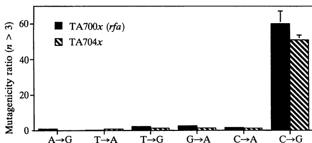
FIG. 7. 5azaC (25 μg)-induced base substitutions.
