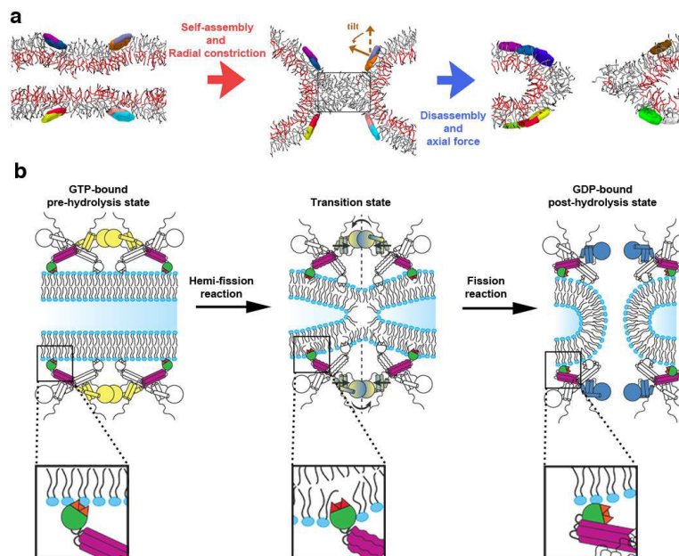
Figure 4. The two stages of dynamin-catalyzed membrane fission
