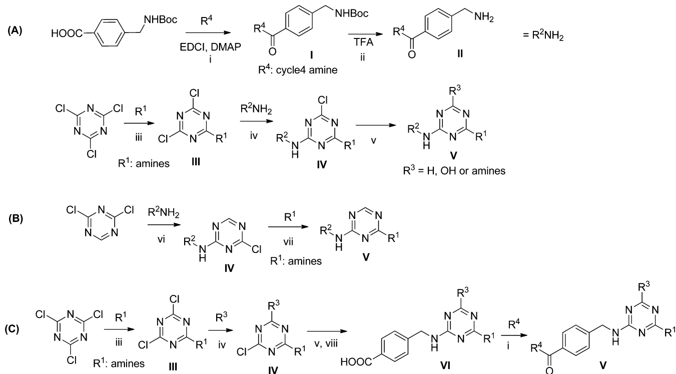
Scheme 1. Synthesis of ADAMTS-4 Off-DNA Hits a
