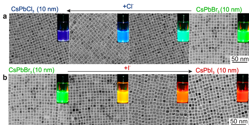
Figure 2. Transmission electron microscopy (TEM) images of \sim 10 nm \text{CsPbX}_3 NCs after treatment with various quantities of (a) chloride and (b) iodide anions. The insets show the evolution of emission colors (under a UV lamp, \lambda = 365 nm) upon forming mixed-halide \text{CsPb}(\text{Br}/\text{Cl})_3 and \text{CsPb}(\text{Br}/\text{I})_3 to fully exchanged \text{CsPbCl}_3 and \text{CsPbI}_3 NCs.
