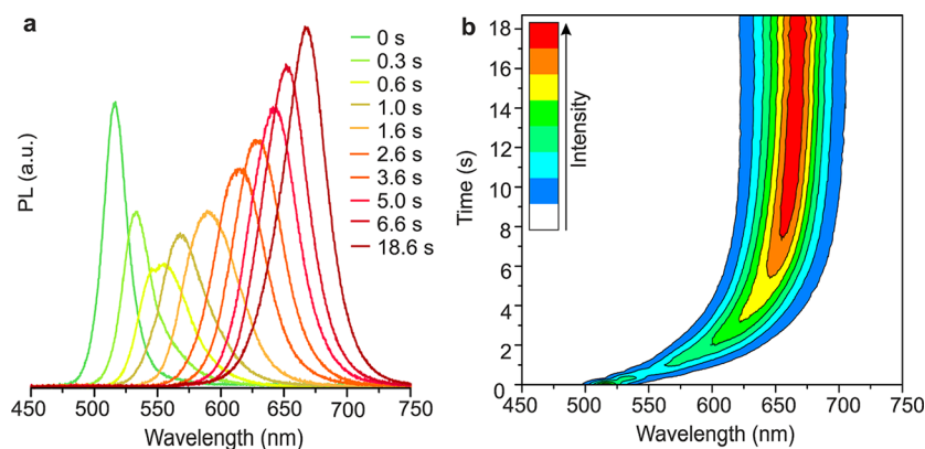
Figure 4. In-situ PL measurements during a CsPbBr 3 to CsPbI 3 NC conversion at 40 °C with [Br]_{parent}/[I]_{incoming} = 1:3 , (a) plotted at specific times during conversion and (b) throughout the complete process (with three spectra acquired per second).
