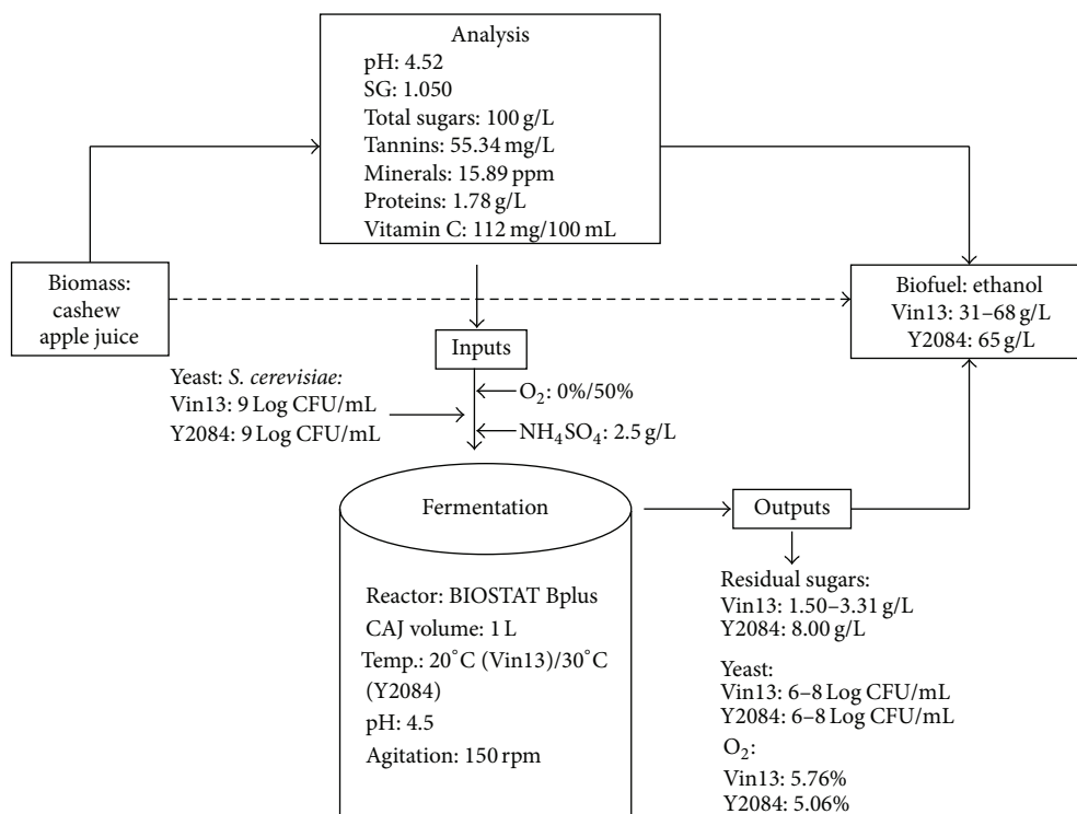
FIGURE 3: Cashew apple juice-ethanol production process.
