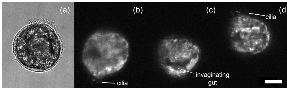
Fig. 4. Images of an optically trapped S. lamarcki larva. (a) Bright field image. (b-d) Three examples of light sheet images, obtained with auto-fluorescent signal from the larva. External (cilia) and internal (invaginating gut) structures of the larva can be identified. Scale bar 20\ \mu\text{m} . See Visualization 2 and Visualization 3 for corresponding bright field and light sheet imaging videos.
