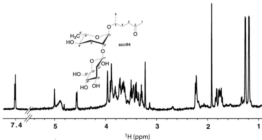
Fig. 3 1D ^1\text{H} NMR spectrum from our study to isolate and identify a component of the mating pheromone of Caenorhabditis elegans (Srinivasan et al. 2008). This spectrum was collected using one of the most sensitive NMR probes available (Brey et al. 2006). Because the pheromone is present in such low concentrations, this spectrum required about 4 million worm equivalents of material. A male C. elegans can detect as little as 2.5 worm equivalents (Kaplan et al. 2011).
