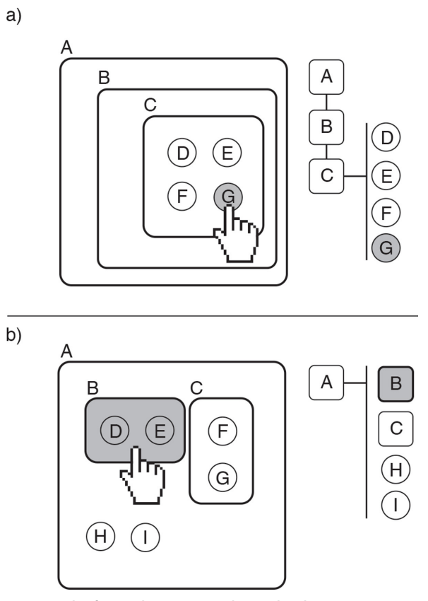
Figure 4 The figure demonstrates hierarchical inspection using the symbolic overview and the the pruned tree. In (a), the user selects protein G from the expanded node within the node-link diagram; this protein is highlighted within the pruned tree visualization, which also provides more information about its siblings (the proteins D, E, and F) and its parent and grandparent nodes (the complexes C, B, and A). In (b), the user selects a complex B in the expanded node, which is displayed in a similar manner in the pruned tree.
