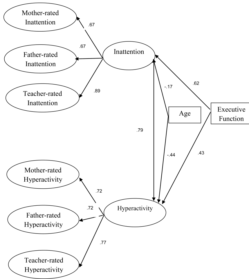
Figure 1. Simplified SEM of Mother, Father, and Teacher ADHD Symptom Ratings Note. All loadings significant at p < .01 .
