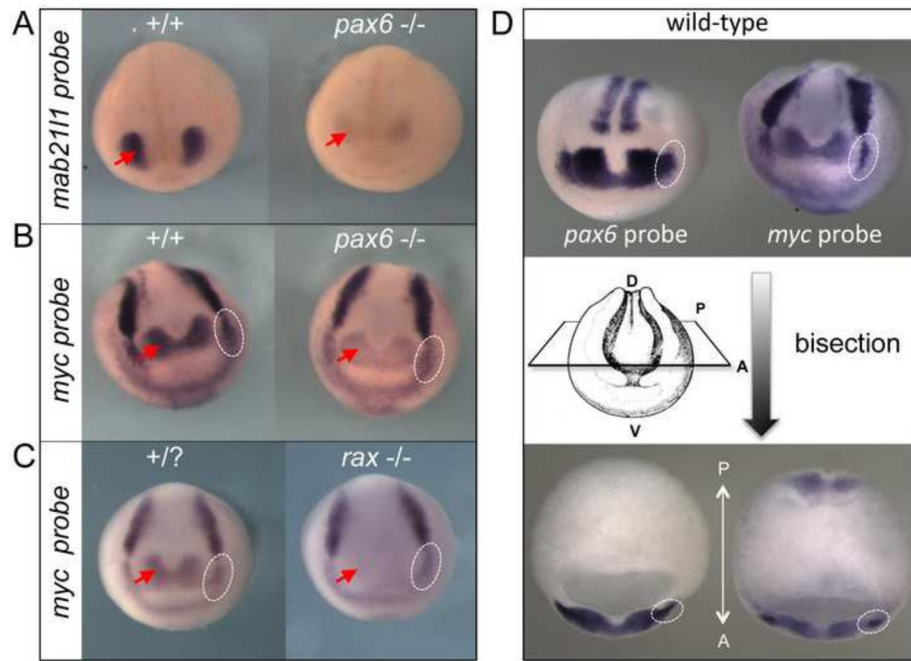
Fig. 6. mab2111 and myc are downstream of pax6 . (A–B) In situ hybridization of wild-type (+/+) and pax6 mutant embryos (-/-, compound heterozygote of complex 1 and 10-kbp inversion mutations, see Table S1 for sequence) at st. 21 (A) or st. 15 (B) with mab2111 (A) or myc (B) probe. Red arrows indicate expression of mab2111 (A) and myc (B) in the eye region. Expression of both genes is reduced in mutants. (C) In situ hybridization of wild-type (+/?) and rax mutant (-/-, see Fish et al., 2014) embryos with myc probe. Note that myc expression in the presumptive retina region (red arrow) is almost completely lost in the rax mutant as reported previously (Fish et al., 2014), whereas in the pax6 mutant myc expression is consistently reduced, but to a lesser extent as shown in (B). White dotted circles show the presumptive lens ectoderm (PLE) region, in which expression of myc is indistinguishable between wild-type and rax mutant embryos. By contrast, expression of myc in the PLE of pax6 mutant is reduced compared to the wild-type embryo (B, white dotted circles). (D) In situ hybridization of wild-type embryos with pax6 (top left) and myc (top right) probes at stage 15. The same embryos are bisected at the level shown schematically, clearly showing the expression of pax6 and myc in the PLE (bottom, white dotted circles).
