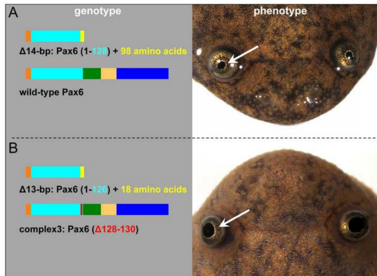
Fig. 9. Combination of truncated Pax6 protein and Pax6 protein with small in-frame deletion causes an aniridia-like phenotype in X. tropicalis froglets. (A) An example of a heterozygous genotype (left) of phenotypically wild-type froglet (right). (B) An example of the compound heterozygous genotype (left) of an aniridia-like froglet (right). All other genotypes of aniridia-like froglets are listed in Table S1.
