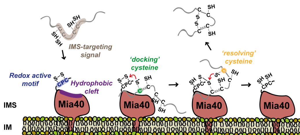
Figure 3. Molecular recognition of substrates containing twin CX 3 C or CX 9 C motifs by Mia40. Precursors containing IMS-targeting signals (ITS/MISS) “slide” onto the hydrophobic binding cleft of Mia40 via hydrophobic interactions. This allows docking of its active cysteine to the CPC motif of Mia40 intermolecularly. The substrate is released when the “resolving” cysteine forms an intramolecular disulfide with the “docking” cysteine.
