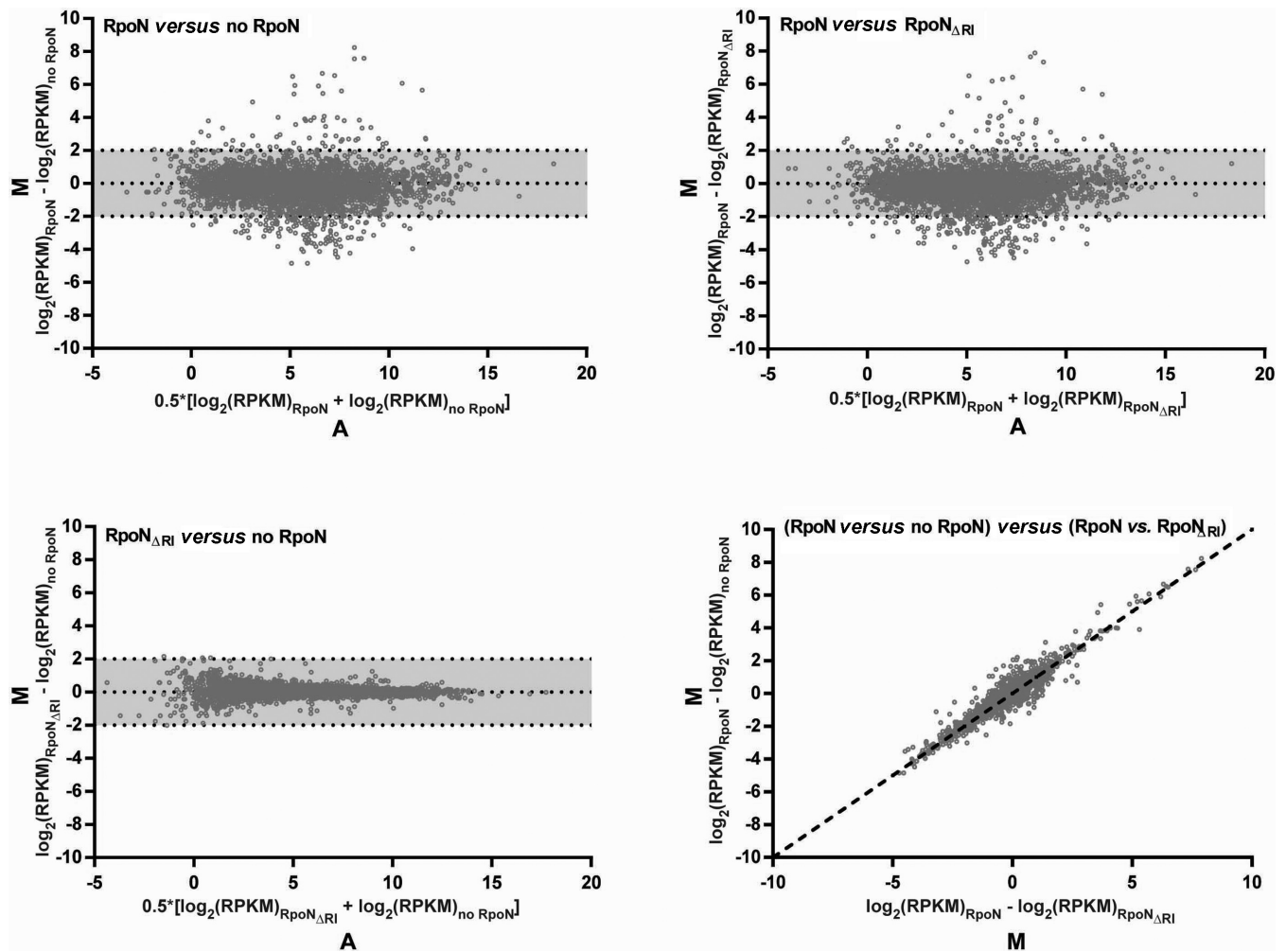
Figure 5. Genome-wide transcriptional profiling by RNAseq revealed no major global bypass transcription by RpoN ΔRI . Shown are MA scatterplots comparing cells with wild-type RpoN to cells with no RpoN (Top left) or RpoN ΔRI (Top right) as well as cells with RpoN ΔRI to cells with no RpoN (Bottom left). M is the difference in number of reads for each gene between a pair of strains expressed as \log_2(\text{RPKM})_{\text{Strain 1}} - \log_2(\text{RPKM})_{\text{Strain 2}} , i.e. values > 0 indicate higher expression in strain 1 while values < 0 indicate higher expression in strain 2. A is the average number of reads of a gene between both strains expressed as 0.5 \cdot [\log_2(\text{RPKM})_{\text{Strain 1}} + \log_2(\text{RPKM})_{\text{Strain 2}}] . Data points within the grey shaded area ( M = \log_2(\text{RPKM}) = \pm 2 ) depict genes less than equal to four-fold differently expressed between the strains. The scatterplot in the Bottom right corner compares the M-values of the Top left and Top right plot showing that the differences in gene expression between cells with wild-type RpoN and no RpoN are similar to the differences in gene expression between cells with wildtype RpoN and RpoN ΔRI (dotted line: y = x ). The data is derived from single sample analysis.
