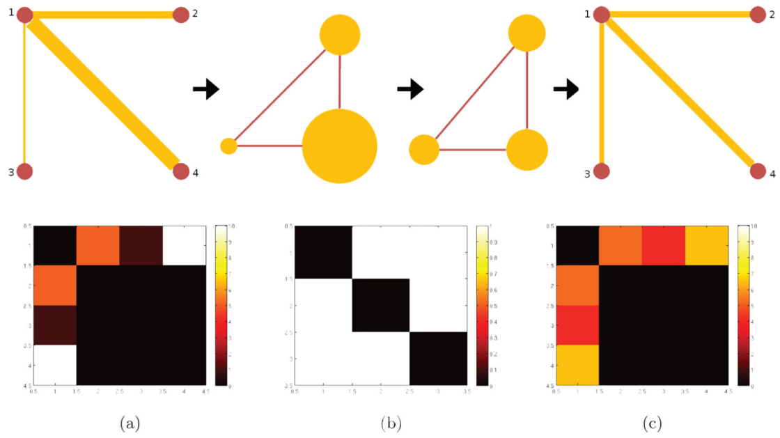
Figure 2. A toy example of graph structure filtering. The top row shows the graph filtering steps: (1) construction of the line graph, (2) smoothing(filtering) the signal on the line graph vertices, (3) reconstructing the filtered graph. The bottom row shows the corresponding adjacency matrices for each step.
