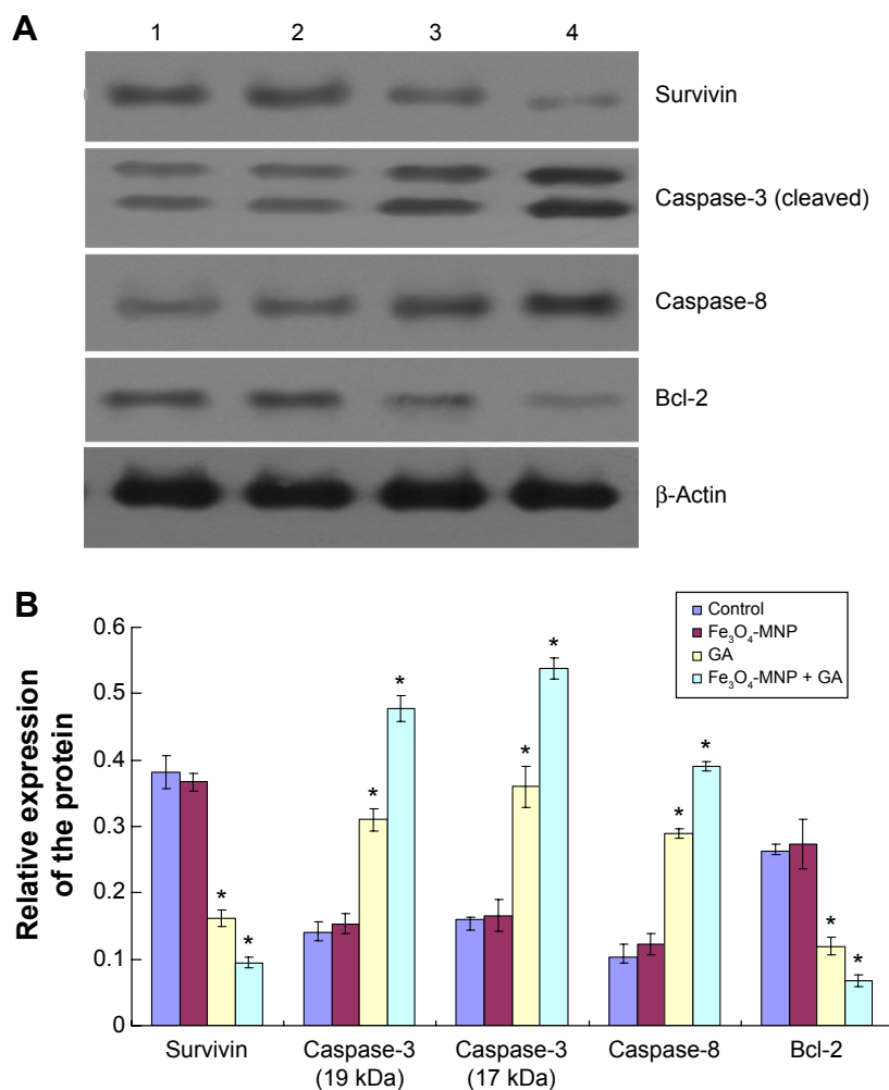
Figure 7 (A) Effect of GA and Fe 3 O 4 -MNP on the protein expression level of survivin, caspase-3, caspase-8 and Bcl-2 in SMMC-7721 cells for 48 h. (1) Control, (2) 20 μg/mL Fe 3 O 4 -MNP, (3) 0.5 μmol/L GA, and (4) 20 μg/mL Fe 3 O 4 -MNP + 0.5 μmol/L GA. (B) Bar graph showing Western blot analysis of survivin, caspase-3, caspase-8, and Bcl-2 in SMMC-7721 cells for 48 h.
