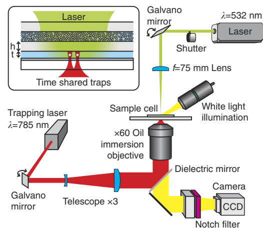
Figure 2 | Experimental setup. An intense green laser ( \lambda = 532 nm) is weakly focused on one side of the sample cell using an f = 75 mm lens. A turbid scattering layer of thickness 20 \mu\text{m} at the entrance of the cell creates a random field distribution inside a light-filled cavity of dimensions \sim (50 \mu\text{m})^3 . From the opposite side, the sample cell is illuminated with a tightly focused near-infrared laser ( \lambda = 785 nm) creating a set of two time-shared optical traps. Both laser beams can be steered by galvano mirrors. A white light source is employed for the broadband illumination of the cell, allowing the tracking of the particles by video microscopy. Different filters are used to spectrally isolate the different optical paths. The interaction potential between the two trapped spheres is obtained by monitoring the thermal Brownian motion inside the optical traps with a digital camera (CCD). The inset shows an enlarged view of the sample cell: Two micron-sized colloidal particles suspended in water are trapped in the centre of a water-filled layer of thickness t = 15 \mu\text{m} . The water layer and the turbid layer are separated by a glass wall of thickness h \approx 20 \mu\text{m} . The dichroic mirror at the bottom of the clear layer reflects > 99\% of the incoming light leading to multiple reflections inside the cavity.
