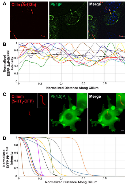
Fig. 1. PI(4)P and PI(4,5)P 2 are present in distinct ciliary compartments (A) IMCD3 cells transfected with EGFP-2×P4M SidM , a PI(4)P sensor, were stained with antibodies against the ciliary protein Arl13b (red) and EGFP (green). Nuclei were marked by DAPI (blue). (B) Normalized EGFP-2×P4M SidM intensity for ten IMCD3 cilia was plotted against normalized distance along the cilium. The black dotted line is the linear regression of all cilia. (C) Cilia of live NIH-3T3 cells were visualized by 5HT 6 -CFP fluorescence (false colored red). PH PLCd1 -EYFP, a PI(4,5)P 2 sensor, accumulated in the proximal ciliary region (false colored green). Scale bar, 5μm. (D) Normalized EYFP-PH PLCd1 intensity for eleven NIH-3T3 cilia was plotted against normalized distance along the cilium and the data fitted to sigmoidal curves. The black dotted line is the average of all curves.
