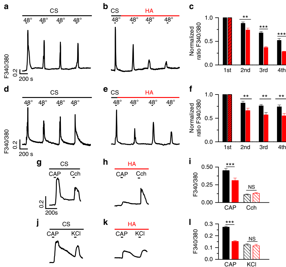
Figure 1 | Inhibition by HA of intracellular calcium responses to heat (48 °C) and 100 nM CAP in HEK-TRPV1-EYFP (+) cells and DRG primary sensory neurons. (a) Intracellular calcium rises evoked in a HEK-TRPV1-EYFP (+) cell by temperature elevations of the bathing solution to 48 °C repeated at 10 min intervals. Cytosolic \text{Ca}^{2+} increases are represented as the ratio of the emission fluorescence intensities at 340 and 380 nm. Notice the development of desensitization. (b) The same experiment as in a but with a HA perfusion, at the end of the first heating stimulus. (c) The normalized ratio of average amplitude between responses evoked by successive heat pulses (indicated in the abscissae axis) in the control solution (CS, black bars) and during perfusion with HA (red bars). Striped red bar represents the average amplitude of the response in the control saline solution for cells treated with HA immediately afterwards. Notice that the inhibition was maximal at 30 min after the onset of the HA perfusion. (d-f) The same protocol as in a-c but performed in cultured adult DRG primary sensory neurons. The inhibitory effect was maximal after 20 min of HA perfusion (third versus first stimuli). (g,h) Intracellular calcium change in a HEK-TRPV1-EYFP (+) cell in response to 100 nM CAP and to 100 \mu\text{M} carbachol (Cch), a compound that activates endogenous muscarinic receptors in HEK293 cells, applied in CS (g) and after exposure to HA initiated 30–60 min earlier (h). (i) The average amplitude of the response to CAP (filled bars) and Cch (striped bars) under perfusion with CS (black, n=68 ) and in the presence of HA (red, n=100 ). (j-k) Intracellular calcium responses of DRG adult cultured sensory neurons to 100 nM CAP and to 30 mM KCl during perfusion with the control solution (j) and with HA (k). (l) The average amplitude of the intracellular calcium responses of DRG neurons to CAP (filled bars) or 30 mM KCl (striped bars) in control solution (black) and in the presence of HA (red). Note that the [\text{Ca}^{2+}]_i increase evoked by membrane depolarization of CAP-sensitive neurons with 30 mM KCl was not altered by HA. The data are represented as the mean \pm s.e.m. Student's t -test: *** P < 0.001 ; ** P < 0.05 ; NS P > 0.5 .
