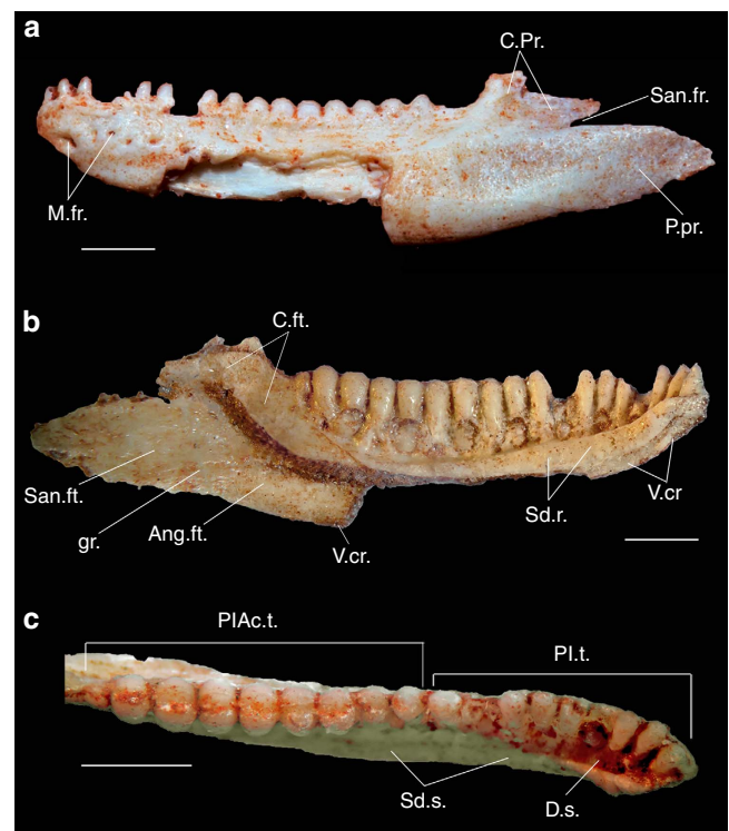
Figure 1 | Holotype of Gueragama sulamericana . CP.V 2187 in (a) labial, (b) lingual and (c) occlusal views. Ang.ft., angular fac; C.ft., coronoid facet; C.Pr., coronoid process; D.s., dental sulcus; gr., groove; M.fr., mental foramina; P.pr., posterior process; Pl.t., pleurodont teeth; PIAc.t., pleuroacrodont teeth; San.fr., surangular foramen; San.ft., surangular facet; Sd.r., subdental ridge; Sd.s., subdental shelf; V.cr., ventral crest of dentary. Scale bars, 2 mm.
