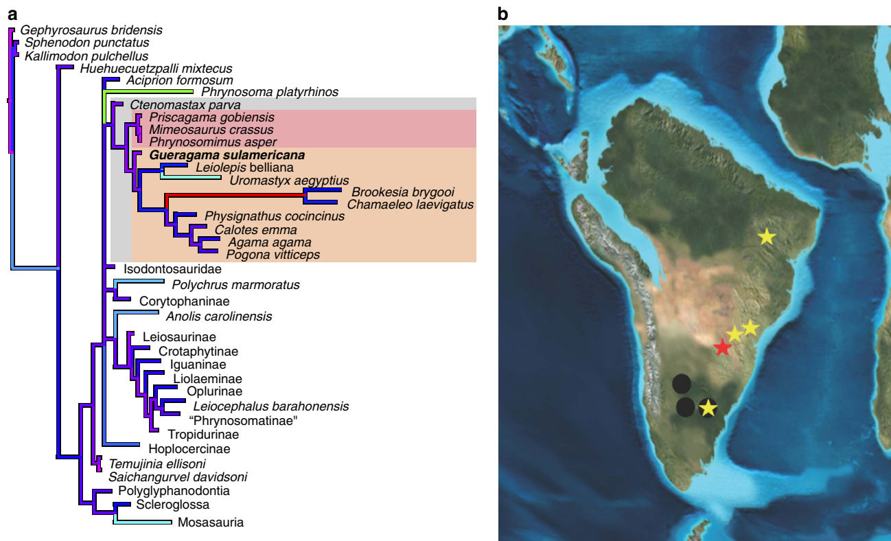
Figure 3 | Phylogenetic position of Gueragama sulamericana among other squamates, and lepidosaur distribution in the Cretaceous of South America.
