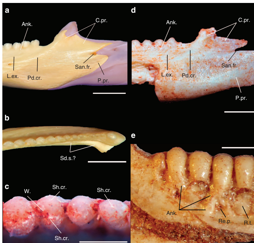
Figure 2 | Details of Gueragama sulamericana and comparisons. Details of the lower jaw of Uromastyx acanthinurus (extant acrodontan—MCZ 27382) in labial (a) and occlusal (b) views. Scale bars, 5 mm. Details on the dentition and dentary of Gueragama sulamericana (CP.V 2,187) in occlusal (c), labial (d) and lingual (e) views. Scale bars, 1 mm. Ank., tooth ankylosis to dentary bone; L.ex., labial excavation on dentary; Pd.cr., posterodorsally ascending crest; Re.p., resorption pits; Re.t., replacement tooth; Sd.s., subdental shelf; Sh.cr., shearing crest; W., mediobasal wear facet.
