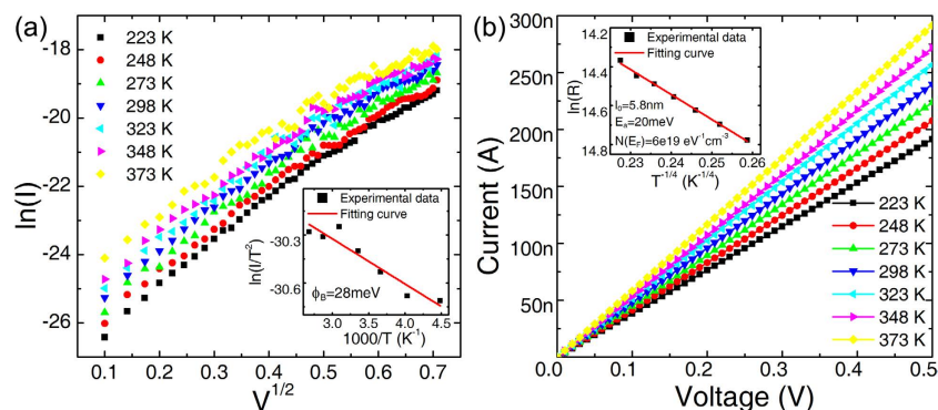
Figure 4. The conductive mechanism of 3D \text{Ta}_2\text{O}_{5-x}/\text{TaO}_y RRAM with graphene edge electrode in (a) HRS and (b) LRS, fitted to Schottky emission model and electron hopping model respectively. Insets show the fitting curves and corresponding fitting parameters.
