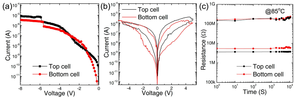
Figure 3. Electrical performance of two-layer 3D \text{Ta}_2\text{O}_{5-x}/\text{TaO}_y RRAM with graphene edge electrode: (a) Forming process of the cells in top and bottom layer which shows a self-compliance property without external device to limit the currents; (b) typical bipolar resistive switching; (c) retention measurement at 85^\circ\text{C} with 1 V read voltage.
