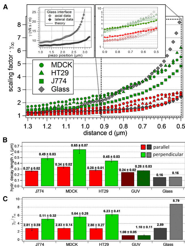
FIGURE 6 Hydrodynamic coupling of a 1 \mu\text{m} bead close to different interfaces. (A) Comparison of \gamma_\perp(d) in green and \gamma_\parallel(d) in red for all cell types and a stiff glass interface, shown in gray diamonds and in the upper left inset together with fits. Data points for all available measurements belonging to the respective cell type were averaged to get the resulting curves. The linear behavior in semi-logarithmic representation (right inset) confirms the nearly exponential decay, highlighted for the case of the MDCK cells. (B) Bar diagram of hydrodynamic decay lengths A_\perp and A_\parallel for all investigated cell types, the GUVs and the glass interface. (C) Summary of the measured values \gamma_{0\perp} and \gamma_{0\parallel} in units of \gamma_\infty = 8.0 \times 10^{-9} Ns/m. Numbers in (B) and (C) are mean values \pm standard deviation. GUV data in (B) and (C) are displayed in darker colors and glass data in gray, where dark gray represents parallel and light gray perpendicular data. To see this figure in color, go online.
