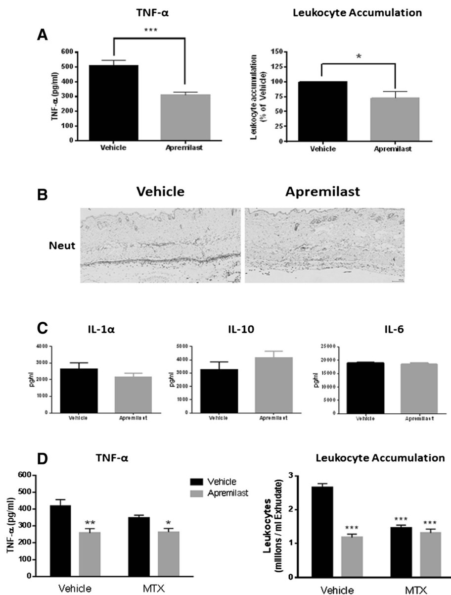
Fig. 2 Apremilast and methotrexate (MTX) prevent inflammation in the air pouch independently. Mice were orally treated with apremilast (5 mg/Kg), and inflammation in the air pouch was induced as described under “Materials and methods”. a TNF-α and leukocyte accumulation were quantified in the exudates of the air pouch. b Immunohistology reveals a decrease in the number of neutrophils ( Neut ) by apremilast treatment. c IL-1α, IL-6 and IL-10 levels were measured in the air pouch exudates with the Luminex multiplex technology. d TNF-α and leukocyte were quantified in the air pouch exudates in mice after weekly intraperitoneal injections of MTX (1 mg/Kg) for 4 weeks prior to apremilast treatment. Data represent mean ± standard error of the mean of at least three independent experiments. Statistical analysis was performed by the Student’s t test or one-way ANOVA, where *** P < 0.001, ** P < 0.01 and * P < 0.05 vs vehicle
