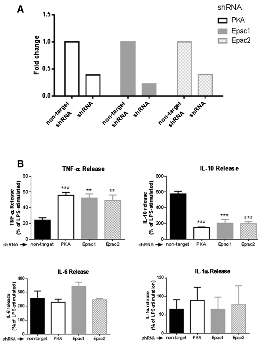
Fig. 6 Effect of Protein kinase A (PKA), Exchange protein directly activated by cAMP (Epac1) and Epac2 knockdown on the action of apremilast. a Transfection of Raw 264.7 cells with shRNA for PKA, Epac1 or Epac2 reduce PKA, Epac1 and Epac2 expression, respectively, as shown by RT-PCR. b PKA, Epac1 and Epac2 knockdown Raw 264.7 cells were incubated with apremilast 100nM for 30 minutes before incubation with or without lipopolysaccharide (LPS) 1 \mu M during 4 h. Levels of TNF- \alpha , IL-10, IL-6 and IL-1 \alpha were analyzed by ELISA or with the Luminex multiplex technology as described under "Materials and methods". Data represent means \pm standard error of the mean of three independent experiments. Statistical analysis was performed by one-way ANOVA with the Bonferroni posttest correction; *** P < 0.001, ** P < 0.01 vs non-target
