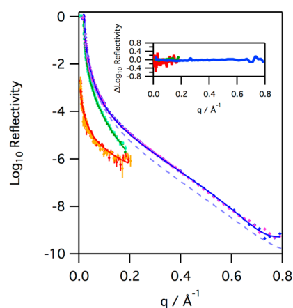
Figure 7. Reflectivity profiles for monolayers of SP-B _{(1-25)} , with an initial surface pressure of 18 \text{ mN m}^{-1} , on \text{H}_2\text{O} buffer (diamonds, blue before ozone, pink after, X-ray data recorded at 21^\circ\text{C} ), \text{D}_2\text{O} buffer (squares, dark green before ozone, light green after, neutron data recorded at 32^\circ\text{C} ), and NRW buffer (circles, red before ozone, orange after, neutron data recorded at 37^\circ\text{C} ) before and after exposure to ozone for 20400 s at \sim 2 ppm (X-ray data), 9072 s at \sim 1 ppm (neutron data with NRW), and 5769 s at \sim 1 ppm (neutron data with \text{D}_2\text{O} ). The solid lines represent the fits to the data before ozone, as described in the text. The dash light blue line represents the reflectivity to X-rays of a clean aqueous buffer interface for reference. The inset shows the change in the reflectivity before and after ozone, specifically the difference between the logarithms of the reflectivity recorded before and after ozone exposure.
