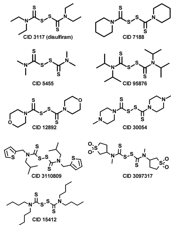
FIG 1 Chemical structures of disulfiram/thiuram disulfide analogs by CID (Pubchem).
