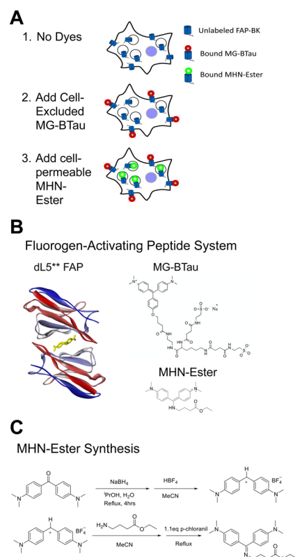
Figure 1. Design of green-inside red-outside (GIRO) labeling (A) schematized paradigm for dye additions. MG-BTau is added first to label surface-exposed FAP; MHN-Ester is then added to label all remaining sites to produce a surface-red internal-green fluorescent signal pattern. (B) Schematic of dL5** FAP, cell excluded MG-BTau, and cell permeable MHN-Ester. Structure shown is dimer of L5** FAP, 33 dL5** is formed by addition of a G4S peptide linker. (C) Condensed schematic of MHN-Ester synthesis (see Supporting Information for detailed synthesis).
