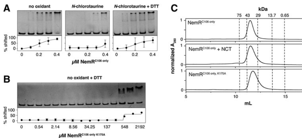
FIG. 4. Disruption of lysine 175 prevents NemR C106 only DNA binding, but does not affect its oligomerization state. (A) EMSAs of the binding of NemR C106 only (0, 100, 200, 300, 400 nM) to nemR promoter DNA ( P_{nemR} , 10 nM) before and after treatment with NCT. To test the reversibility of oxidative inactivation, NCT-oxidized NemR C106 only was incubated with the thiol reductant, DTT (5 mM). Representative gels are shown along with quantification results (mean \pm SD, n=3 ). (B) EMSA of the binding of NemR C106 only, K175A to 10 nM P_{nemR} DNA in the presence of 5 mM DTT (mean \pm SD, n=3 ). Concentration of NemR is plotted on a log 2 scale. (C) Size exclusion chromatography was used to compare the oligomeric state of reduced and oxidized NemR C106 only and reduced NemR C106 only, K175A . Dotted lines indicate elution volume of protein standards of known molecular weight. EMSA, electrophoretic mobility shift assay.
