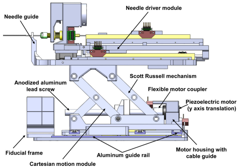
Fig. 4. A side view of the 3-DOF needle driver module providing cannula translation and rotation (2-DOF) and stylet translation (1-DOF) and the 3-DOF actuated Cartesian stage module.
