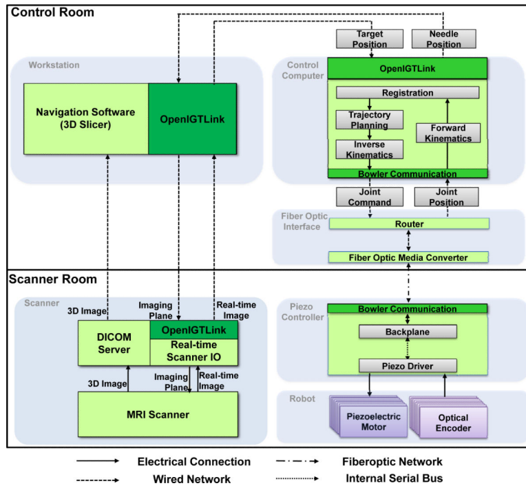
Fig. 2. System architecture and data flow of the robotic system. Six modules are shown in gray block and OpenIGTLink is used to exchange control, image and position data.
