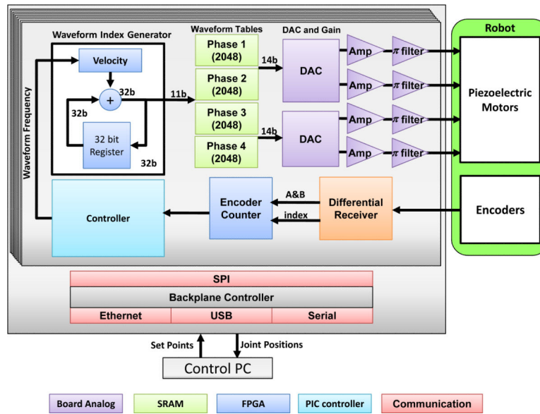
Fig. 5. Block diagram of the system components of each piezoelectric motor driver board. An FPGA is configured as a waveform synthesizer generating the four phases of the drive signal which are passed to a linear amplifier stage with integrated filtering.
