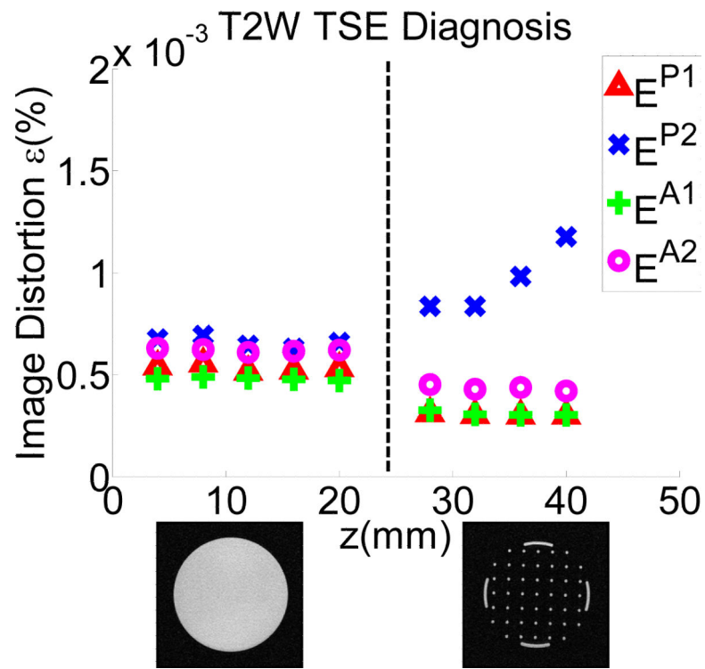
Fig. 12. Passive (P) and Active (A) image deterioration factor \varepsilon variation due to the present and motion of the robot.
