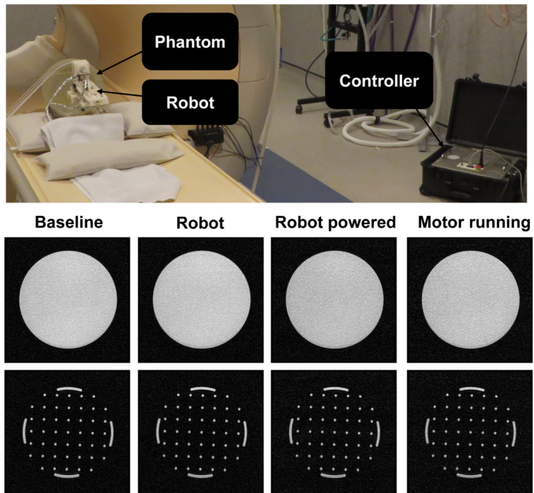
Fig. 10. (First row) The robot prototype configuration in a 3-Tesla MRI scanner with a feature-rich PIQT phantom for the evaluation studies. (Second row) Representative T1-weighted fast field echo images of the cylindrical cross section for each of four configurations. (Third row) Corresponding T1-weighted fast field echo images of the arch/pin cross sections.
