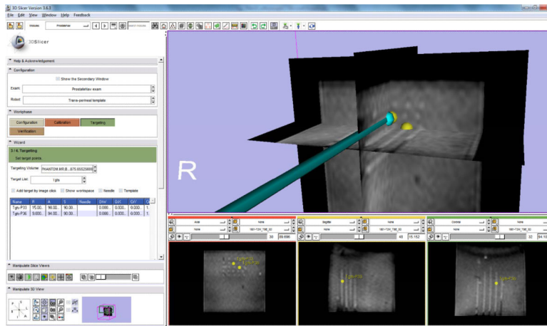
Fig. 9. The clinical GUI integrated inside 3D Slicer shows a virtual needle whose position was streamed from control software, was inserted to move to the selected targets (shown as yellow spheres) during needle placement accuracy evaluation. The needle tracks were visualized inside the MRI volume. The first column of the bottom sub-figures shows the 5 \times 5 needle tracks.
