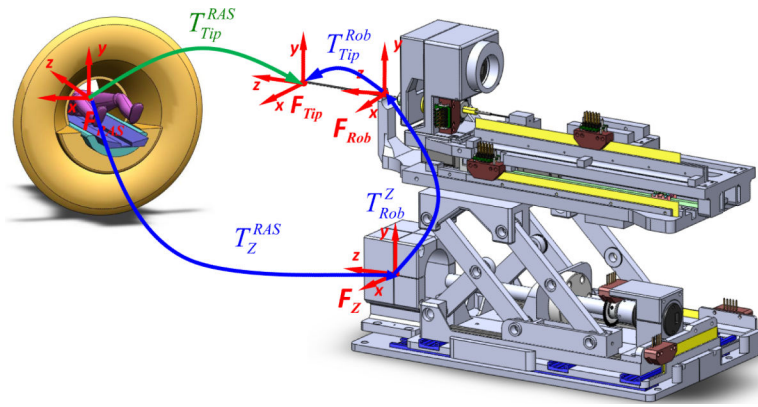
Fig. 7. Coordinate frames of the robotic system for registration of the robot to MR image space, robot kinematics and encoded needle insertion.
