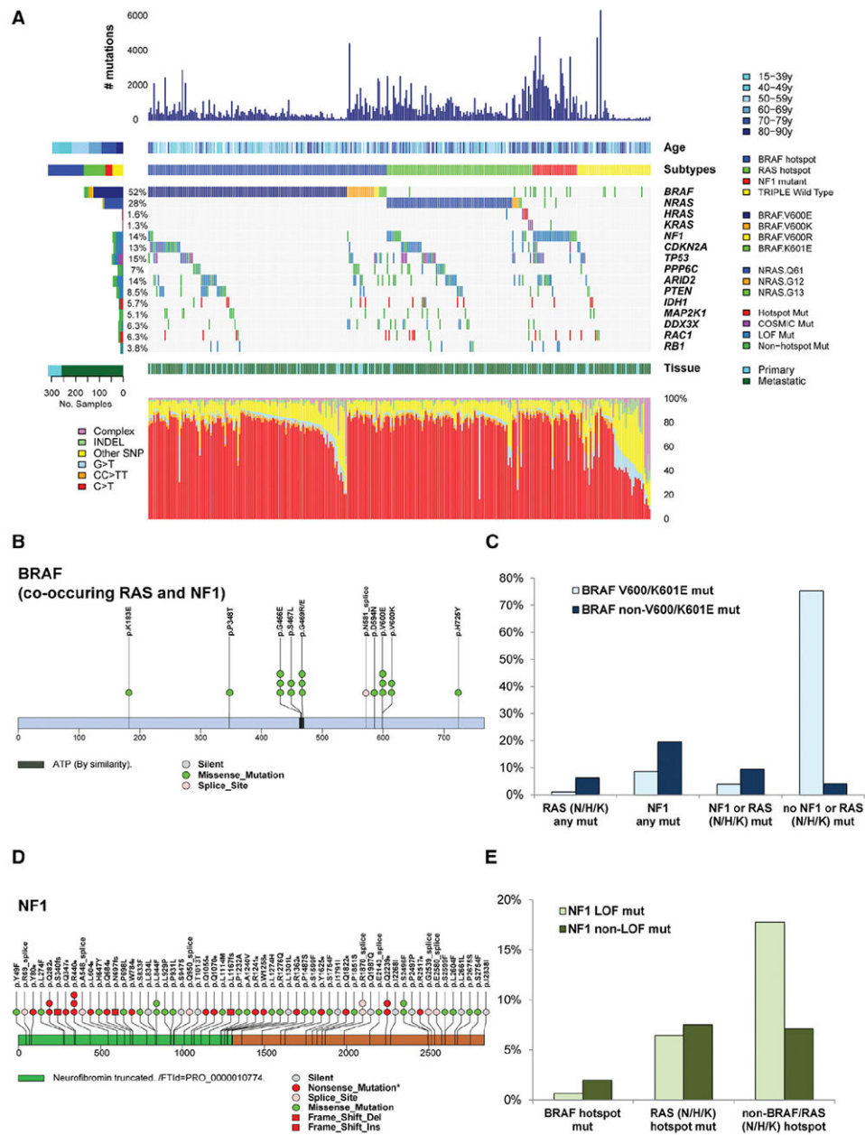
Figure 1. Landscape of Driver Mutations in Melanoma
