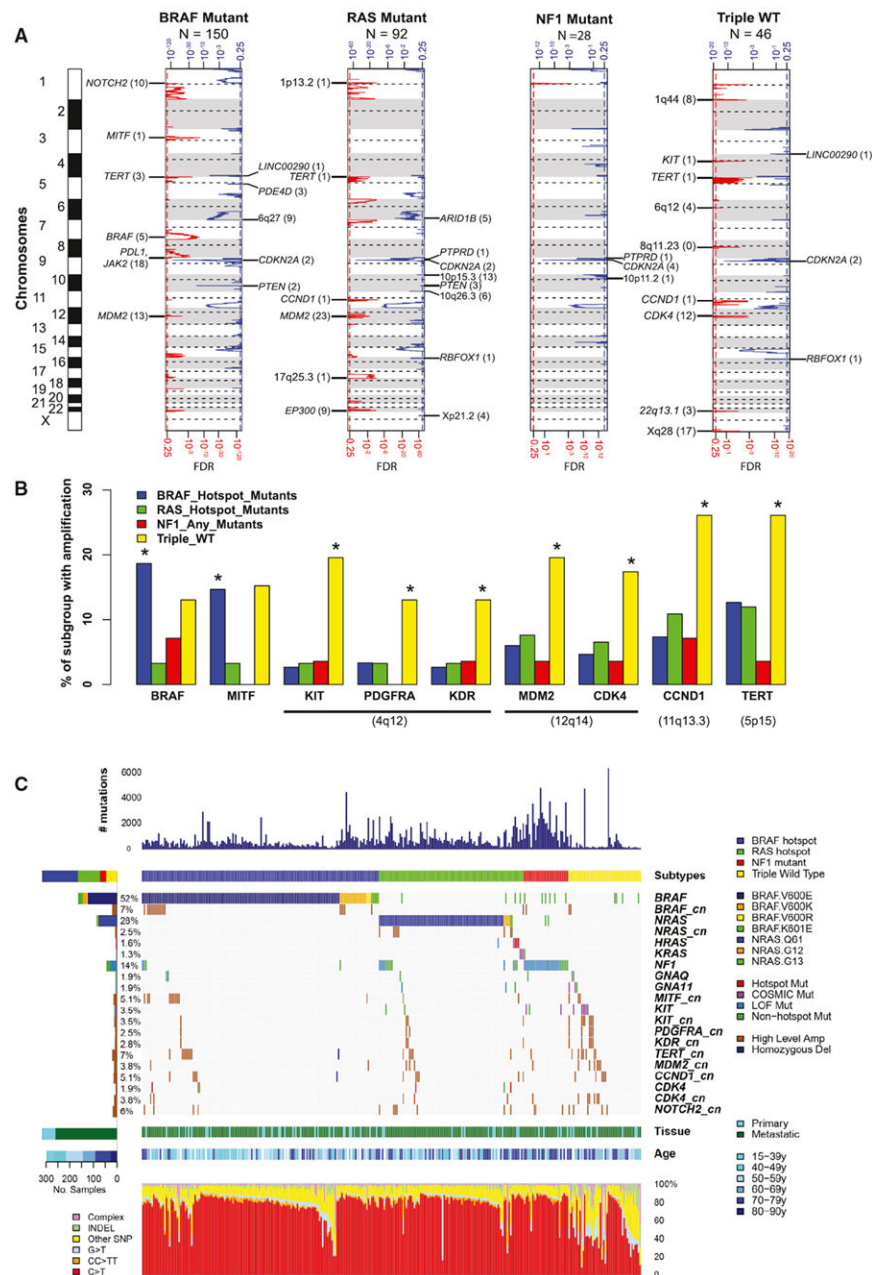
Figure 2. Landscape of Copy-Number Alterations in Melanoma
