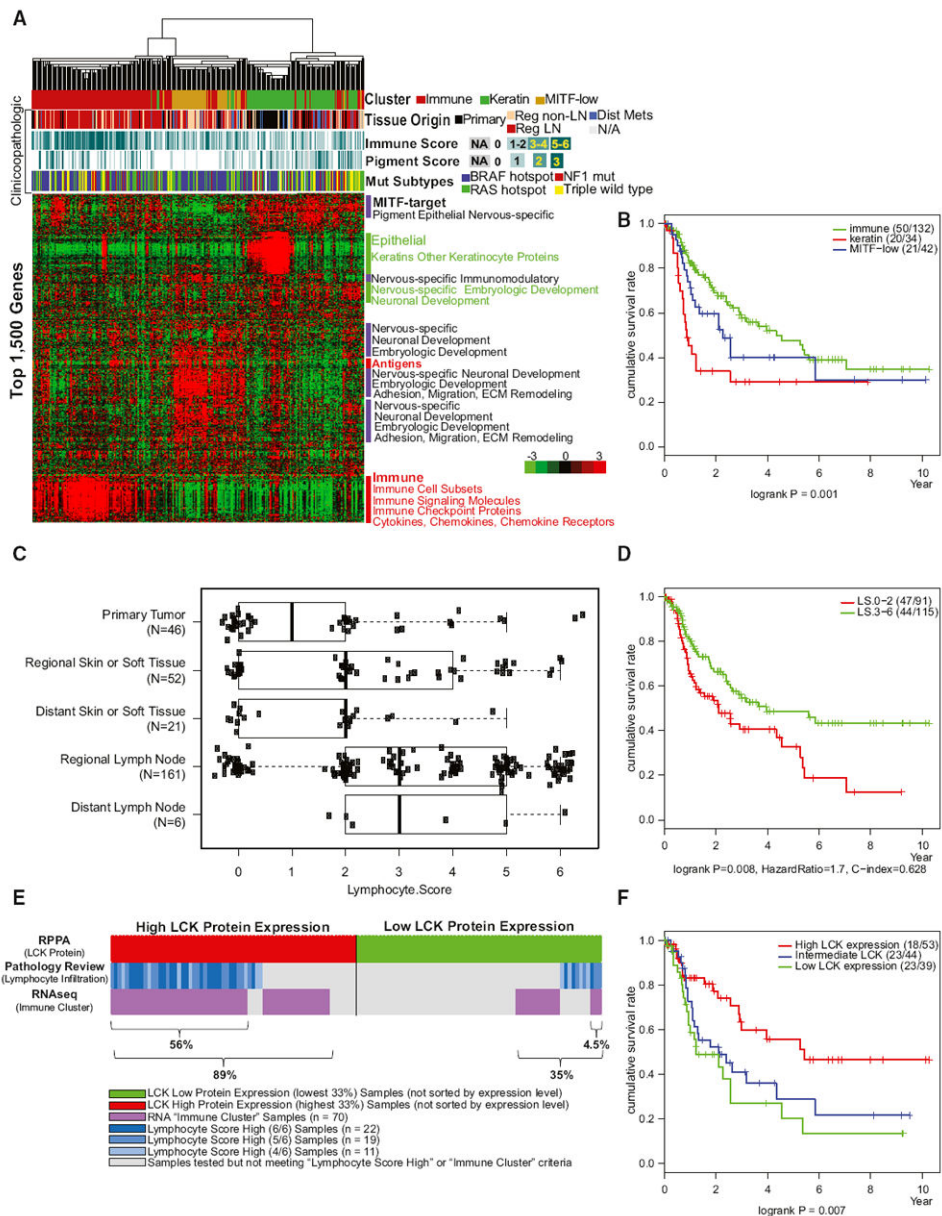
Figure 5. Integrative Analysis across Multiple Molecular Data Platforms Provides Insights into the Biology and Prognostic Significance of Immune Infiltrates in Cutaneous Melanoma (A and B) (A) Unsupervised clustering of 329 melanoma samples using the top 1,500 genes showing the maximum absolute deviation identify three clusters defined as “immune-high,” “keratin-high,” and “microphthalmia-associated transcription factor (MITF)-low” based on gene function of discriminatory mRNAs and (B) post-accession survival curves for RNA subgroups. (C) Distribution of lymphocytic scores determined by histopathology analysis according to sample type (described in detail in the Supplemental Experimental Procedures). (D) Post-accession survival curves for high and low lymphocytic infiltration scores.
