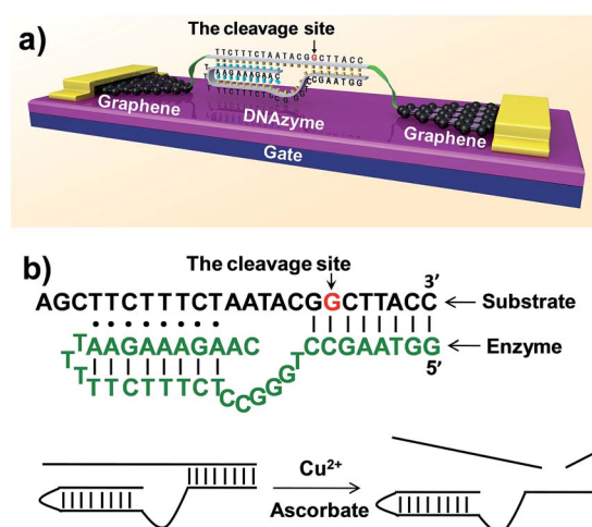
Fig. 1 (a) Schematic representation of graphene–DNAzyme junctions. (b) The structure of the Cu 2+ -sensitive DNAzyme and corresponding catalytic activity. The DNA substrate has been functionalized by amines on both ends for molecular connection (see the ESI†). The cleavage site is indicated by an arrow.
