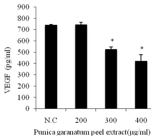
Fig. 5. ELISA demonstrated decreased levels of VEGF in the culture medium at 300 and 400 µg/ml after 24 h incubation. Data are presented as means \pm SD of three experiments. *, P < 0.05 .
