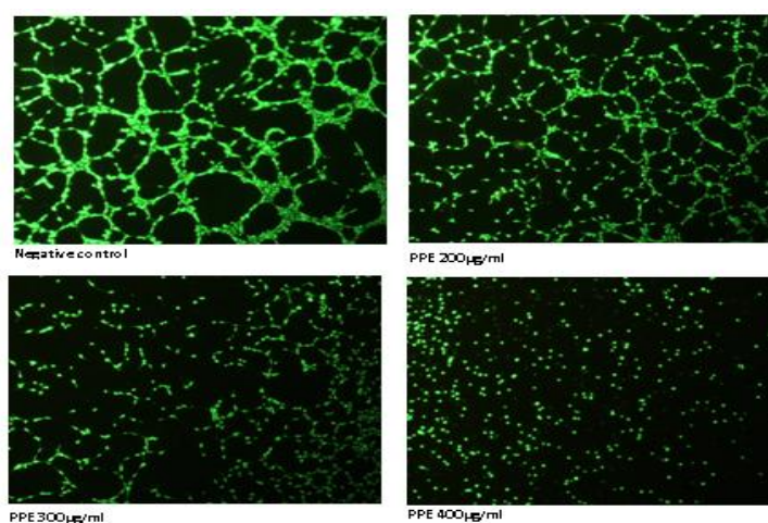
Fig.2. Inhibitory effect of pomegranate peel extract on tube formation of HUVECs. HUVECs were plated on the wells coated with 100 µl of Matrigel basement membrane matrix. After 24 h treatment with different doses of PPE, the cells were stained with calcein and photographed with a Nikon camera attached to a fluorescent microscope at ×10 magnification.
