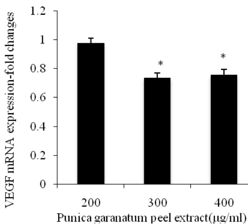
Fig.4. Quantitative analysis of mRNA expression of VEGF in HUVEC by Quantitative real time RT-PCR (Taqman). Total RNA were extracted from HUVEC in medium containing different treatments. The relative expression of VEGF were normalized to GAPDH levels measured in the same RNA preparation. Data shown are from three independent experiments analyzed in duplicate.
