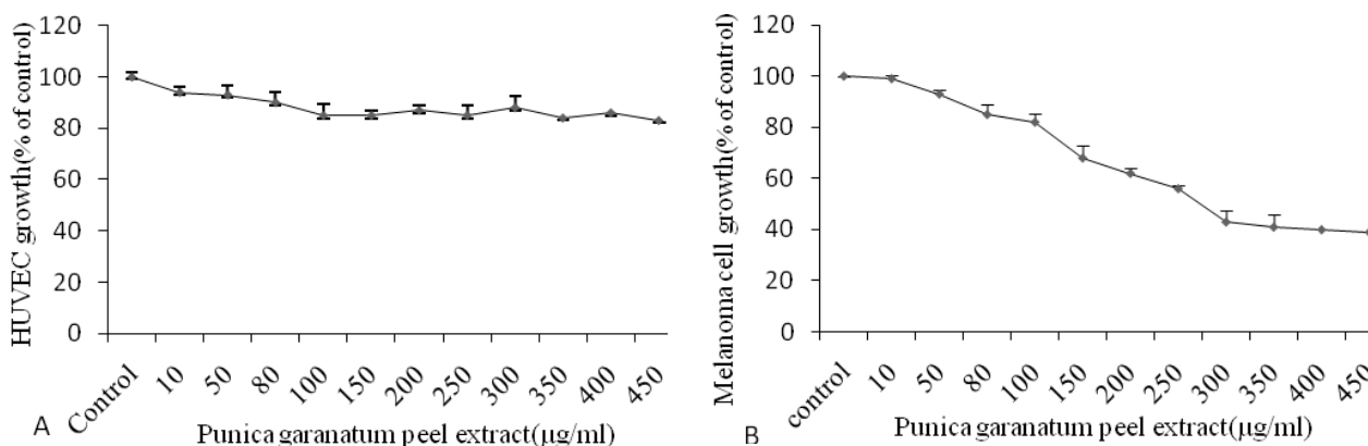
Fig.1. The effects of PPE on cell viability. As detailed in Materials and methods, A; C554 HUVECs, B; B16F10 melanoma cells were treated with PPE and the viability of cells was determined by the MTT assay. The data are expressed as the percentage of cell viability compare to control.
