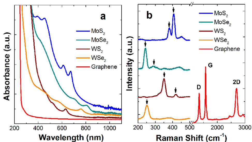
Figure 2. (a) UV-visible spectra of the TMDC (MoS 2 , MoSe 2 , WS 2 , and WSe 2 ) and graphene dispersions. (b) Raman spectra of the dried TMDC and graphene films.
