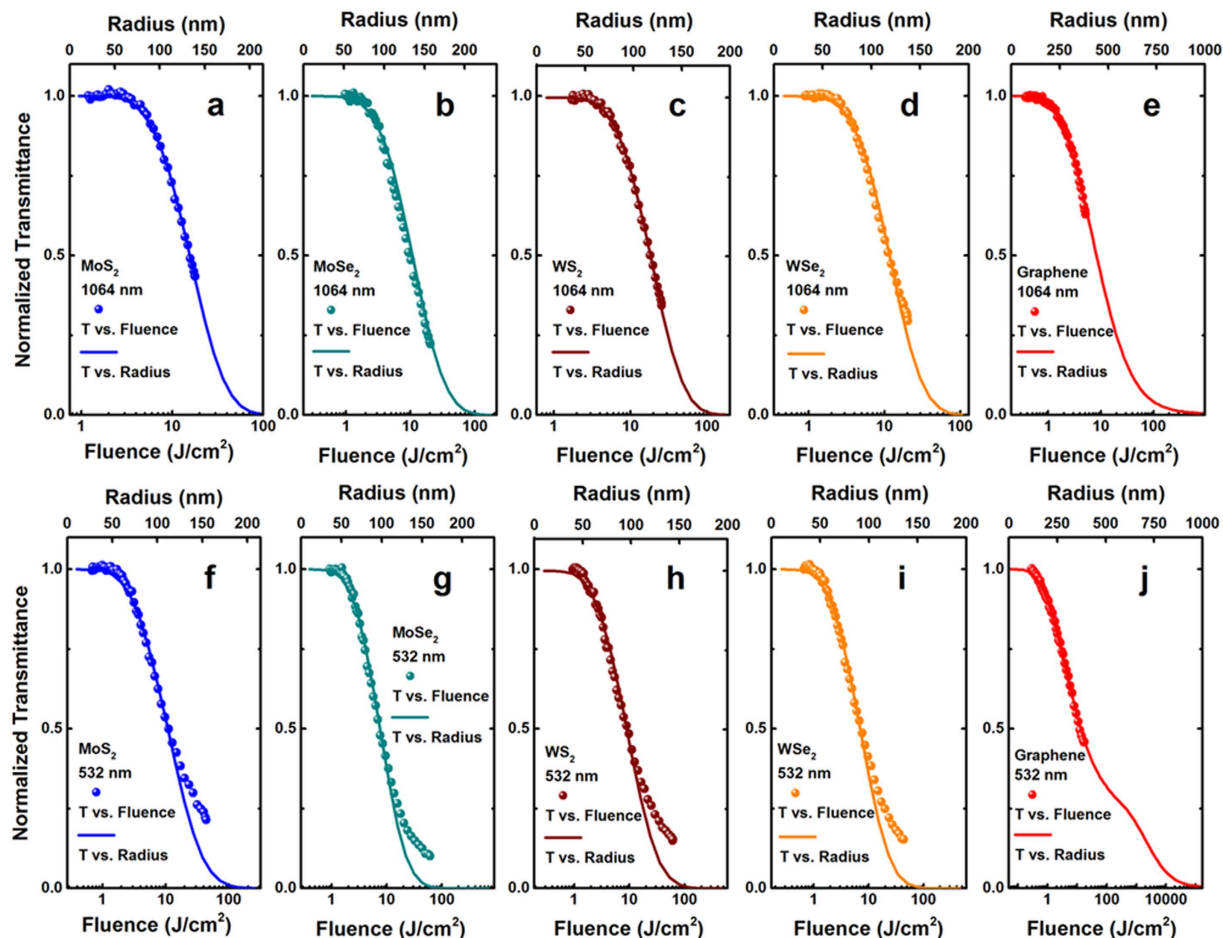
Figure 7. Normalized transmittance as a function of input laser fluence (solid dots) and the radius of micro-bubbles (solid line) for the nanosheet dispersions at 1064 (top row) and 532 nm (bottom row).
