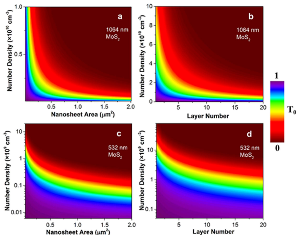
Figure 6. Linear transmittance mapping of MoS 2 dispersions in 10 × 10 mm quartz cuvette at 1064 and 532 nm nanosecond laser pulses. (a,c) Variation in nanosheet number density and area with a constant layer number of 5. (b,d) Variation in nanosheet number density and layer number with a constant area of 0.04 μm 2 . The color bar represents the linear transmittance.
