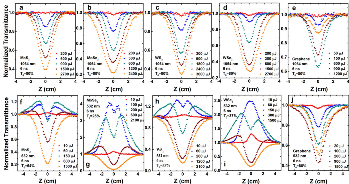
Figure 3. Typical open-aperture Z-scan data with normalized transmittance as a function of the sample position Z for the MoS 2 (a,f), MoSe 2 (b,g), WS 2 (c,h), WSe 2 (d,i), and graphene (e,j) dispersions in NMP at 1064 and 532 nm, respectively, with different incident laser pulse energy.
