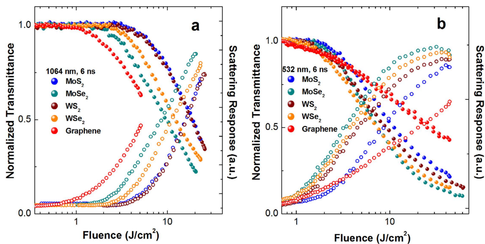
Figure 4. Normalized transmittance (solid circles) and scattering response (open circles) of these nanosheet dispersions at (a) 1064 and (b) 532 nm, respectively.
