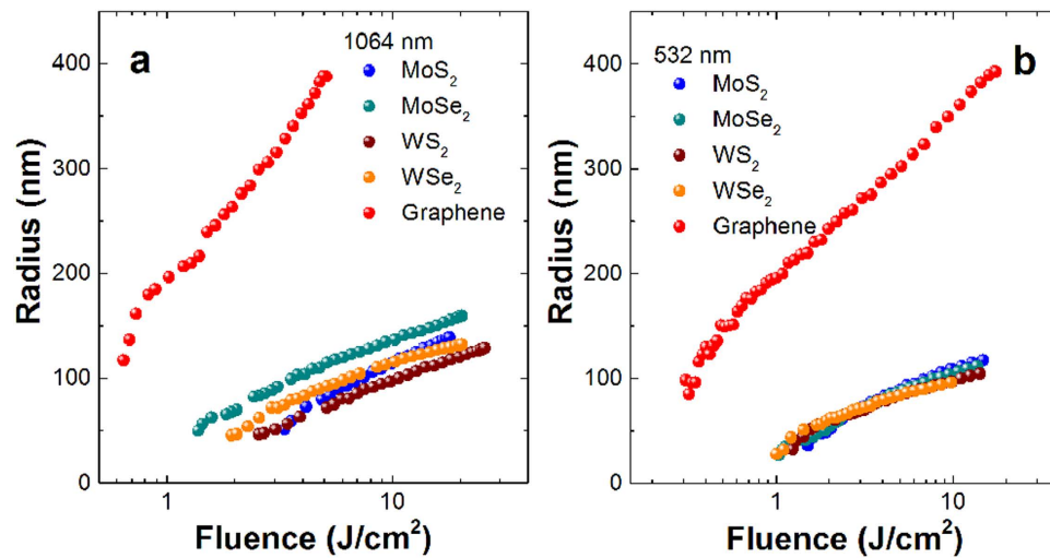
Figure 8. The radius of micro-bubbles variation with the input laser fluence for the nanosheet dispersions at (a) 1064 and (b) 532 nm, respectively.
