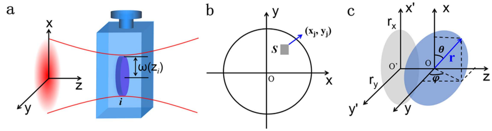
Figure 5. (a) A piece of slab and (b) a nanosheet as a model to explain the calculation process. (c) The schematic to calculate the projected area at xy plane of a nanosheet placed with angles of \theta and \varphi in o-xyz coordinate system.
