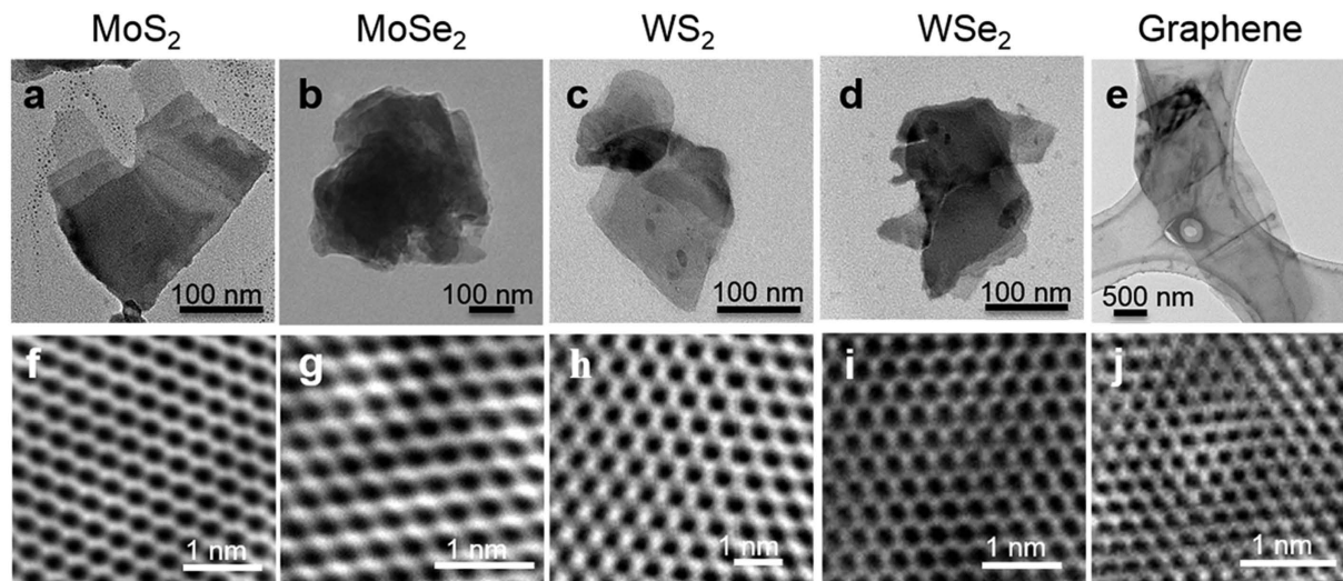
Figure 1. Low-resolution TEM images (top row) and high-resolution TEM images (bottom row) of the MoS 2 , MoSe 2 , WS 2 , WSe 2 , and graphene nanoflakes.
