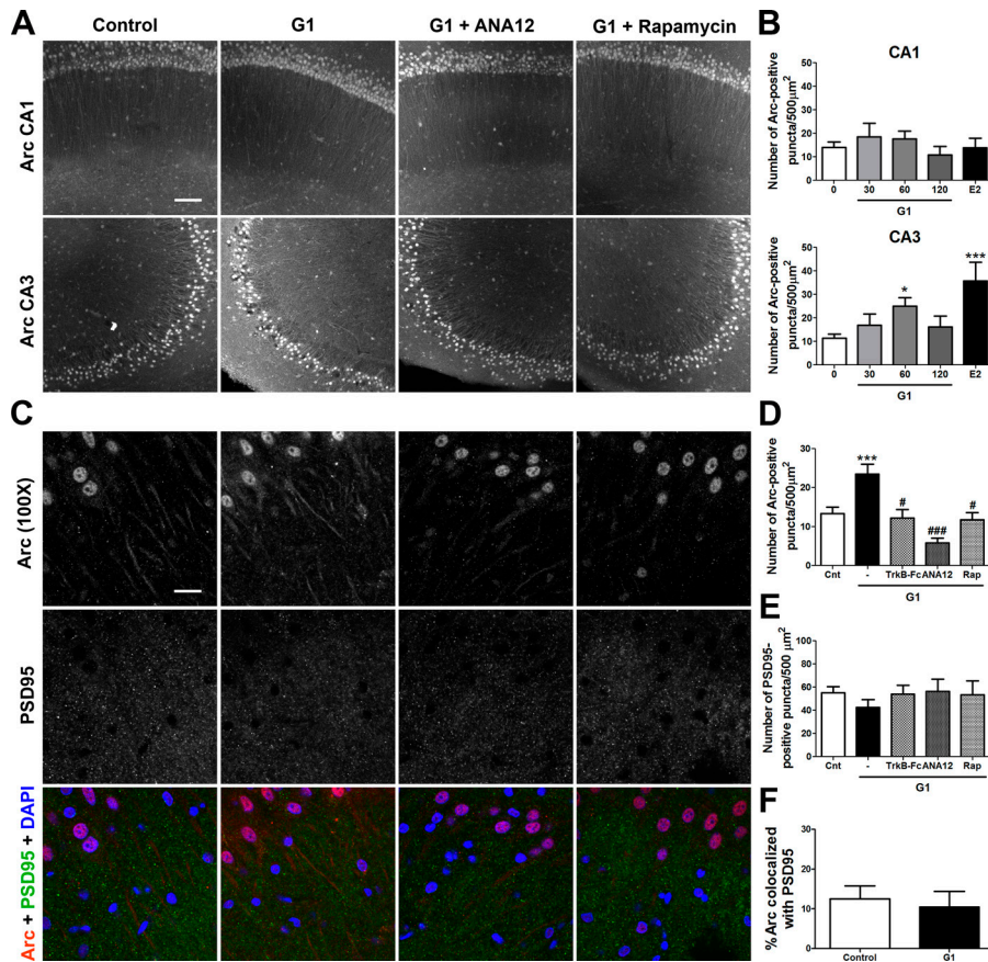
Figure 4. G1 stimulates mTOR-dependent Arc synthesis in CA3 through BDNF release. Hippocampal slices were pretreated with DMSO/lgG-Fc (Cnt), TrkB-Fc, ANA-12, or rapamycin, and then incubated with G1 or E 2 for an additional 60 min or the indicated times. (A) Representative images of Arc immunostaining in CA1 and CA3 under various experimental conditions. Bar, 100 µm. (B) Quantification of density of Arc-positive puncta in CA1 stratum radiatum (CA1sr) and CA3sr. *, P < 0.05; ***, P < 0.001 versus control (n = 3–16, one-way ANOVA). (C) High-magnification images of CA3 from slices double-stained for Arc (red) and PSD95 (green) along with DAPI (blue). Bar, 20 µm. (D and E) Quantification of the density of Arc (D)- and PSD95 (E)-positive puncta in CA3sr. ***, P < 0.001 versus control; #, P < 0.05; ###, P < 0.001 versus G1 (n = 6–29, one-way ANOVA). (F) Percentage of Arc-positive puncta that colocalized with PSD95 (M1 coefficient, n = 11–12). Error bars indicate means ± SEM.
