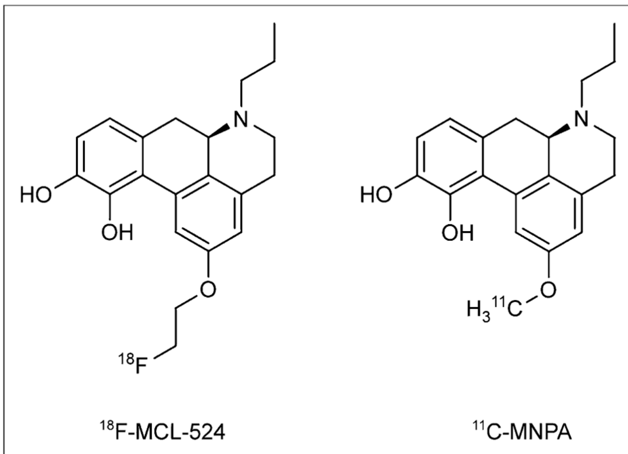
FIGURE 1. Chemical structures of ^{18}\text{F} -MCL-524 and ^{11}\text{C} -MNPA.
