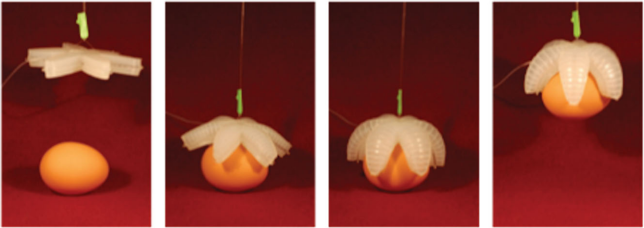
Figure 5. A starfish may not use its appendages to grip objects, but its form inspires mechanical structures that do. Pneumatically actuated soft robotic grippers, which resemble the shape of a starfish, can gently pick up and release an uncooked egg and other fragile, irregularly shaped objects with ease [22].
