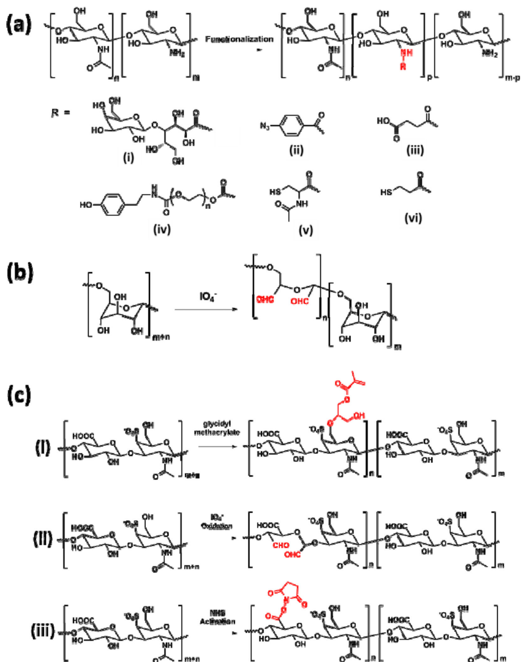
Figure 3. Representative chemical structures of polysaccharide-based sealants. (A) Deacetylation of chitin generates chitosan with different degrees of acetylation, and various chemically modified chitosan derivatives are obtained by reacting chitosan with (i) lactobionic acid, (ii) 4-azidobenzoic acid, (iii) succinic anhydride, (iv) PEG oligomers, (v) N -acetylcysteine, and (vi) 3-mercaptopropionic acid at the amine site [51–57]. (B) Preparation of aldehyde-containing dextran via selective partial oxidation by periodide [60, 61]. (C) Chemical modification of chondroitin sulfate to introduce (i) methacrylate groups via reacting with
