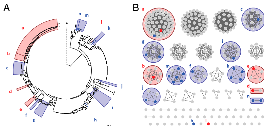
Fig. 1. Diversity of phosphonate biosynthesis in Actinobacteria. (A) Maximum-likelihood phylogeny of actinomycete PepM s using methylisocitrate lyase as the outgroup (*). Complete labeling of strain names is provided in SI Appendix, Fig. S1 . (B) Network diagram of phosphonate gene clusters. In both diagrams, highlighting indicates clades and strains containing pathways for previously described phosphonates (blue) and those phosphonates newly isolated in this study (red). Groups encoding known phosphonate natural products are as follows: a, hydroxynitrilaphos; b, phosphonocystoximate; c, phosphonothrixin; d, valinophos; e, argolaphos; f, dehydrophos; g, fosfazinomycin; h, fosmidomycin; i, plumbemycins and phosacetamycin; j, FR-900098; k, phosphinothricin peptides; l, DMPT; m, fosfomycin; n, 2-hydroxyethylphosphonate polyglycans. Phosphonate gene clusters are available ( www.igb.illinois.edu/labs/metcalf/gcf/Phosphonates.html ).
