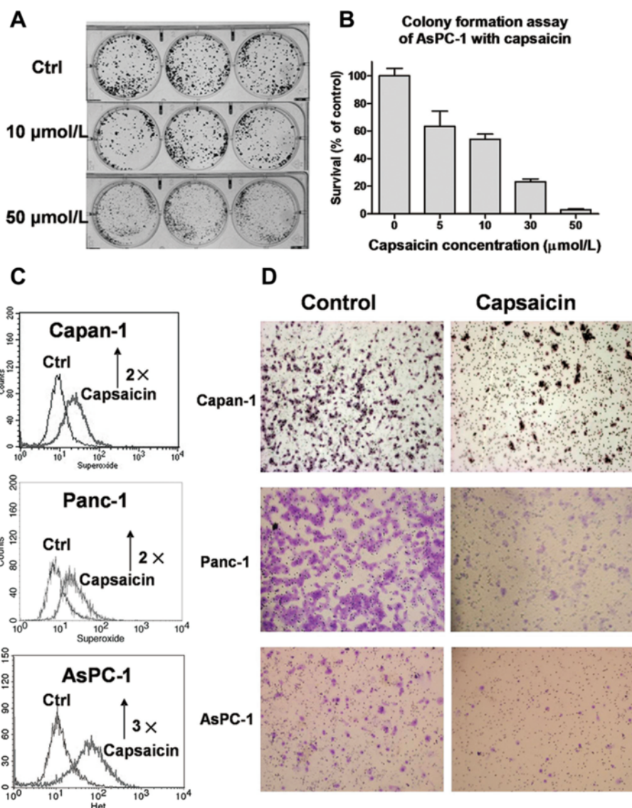
Figure 4 In vitro antitumor activity of capsaicin against the pancreatic cancer cell lines. A , equal numbers of AsPC-1 cells were seeded in 6-well plates in triplicates and incubated with various concentrations of capsaicin (10 and 50 μmol/L) for 14 days. The cells were then fixed, stained, and photographed. B , quantitative analysis of cytotoxic activity of capsaicin in AsPC-1 cells analyzed by colony formation assay. The data are shown as the mean ± SD of 3 experiments. C , the treatment with 30 μmol/L capsaicin for 24 hours induced a 2- to 3-fold increase of cellular superoxide in naturally occurring pancreatic cancer Capan-1, Panc-1, and AsPC-1 cells. D , effect of capsaicin on the invasion of naturally occurring pancreatic cancer cells analyzed by BD BioCoat Chamber as described in the Methods section. Cells were seeded onto the chamber insert with or without 30 μmol/L capsaicin treatment. After 24 hours of treatment, cells that had migrated to the lower surface of the insert were subjected to staining and photographed (magnification, ×400). Ctrl, control.
