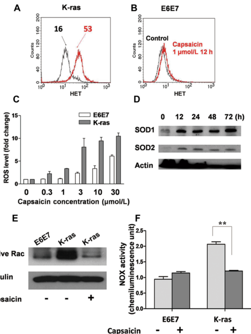
Figure 2 Capsaicin caused preferential reactive oxygen species (ROS) accumulation and selectively inhibited NOX activity in K-ras -transformed E6E7 cells. A , incubation with 1 μmol/L capsaicin for 12 hours caused tremendous ROS accumulation in K-ras -transformed cells as compared with untreated K-ras -transformed cells (superoxide mean level, 16 vs. 53). B , the same treatment caused a minimum effect on ROS production in E6E7 cells as compared with untreated parental E6E7 cells (superoxide mean level, 8 vs. 9). C , the dose-dependent increase in superoxide generation induced by capsaicin in parental and K-ras -transformed E6E7 cells. D , treatment with 10 μmol/L capsaicin caused a significant increase in both SOD1 and SOD2 in K-ras -transformed cells. E , total cell lysates of untreated parental E6E7 cells, untreated K-ras -transformed E6E7 cells, and K-ras -transformed E6E7 cells treated with 10 μmol/L capsaicin for 12 hours were pulled down with nucleotide-free Rac1 G15A agarose beads. The precipitated active Rac was detected by anti-Rac-GEF antibody. F , E6E7 and K-ras -transformed cells were pretreated with 10 μmol/L capsaicin for 12 hours. NOX activity was measured in the presence of 100 μmol/L NADPH by lucigenin-derived chemiluminescence in the plasma membrane fraction of parental and K-ras -transformed E6E7 cells, with or without capsaicin treatment. The values are shown as the mean ± SD. **, P < 0.01.
