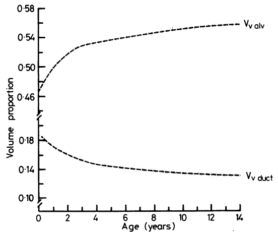
Fig 5 Exponential regression equations for the volume proportion of alveolar duct air ( V_{v\text{ duct}} ) and volume proportion of alveolar air ( V_{v\text{ alv}} ) drawn for boys (mean \pm 1 SE).
