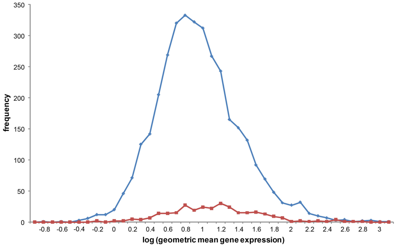
Fig. 3. Frequency histogram of relative gene expression for human housekeeping genes Conserved maternal transcripts (COMATs, red line) tend to have a higher gene expression (measured reads per kb per million mapped reads, RPKM) than non-COMATs (blue). However, COMATs still represent several orders of magnitude of gene expression. Gene expression data from Eisenberg & Levanon (2013).
