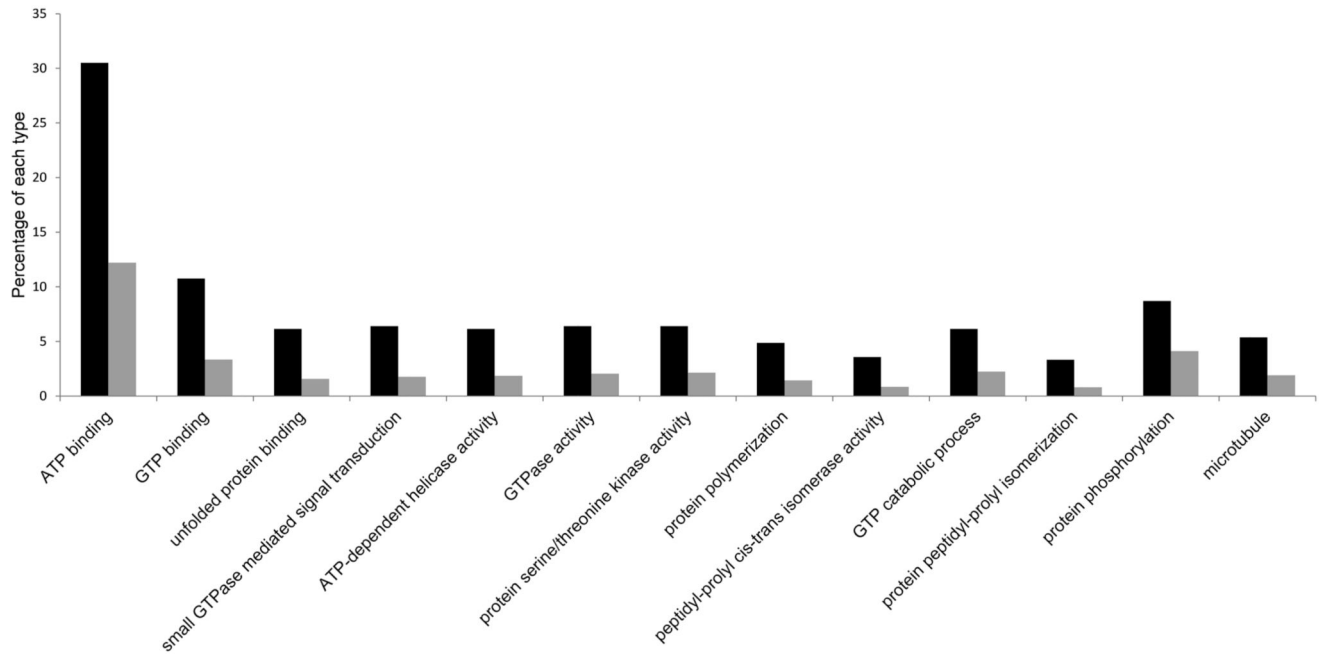
Fig. 1. Enrichment of Gene Ontology terms in the conserved maternal transcript (COMAT) subset
