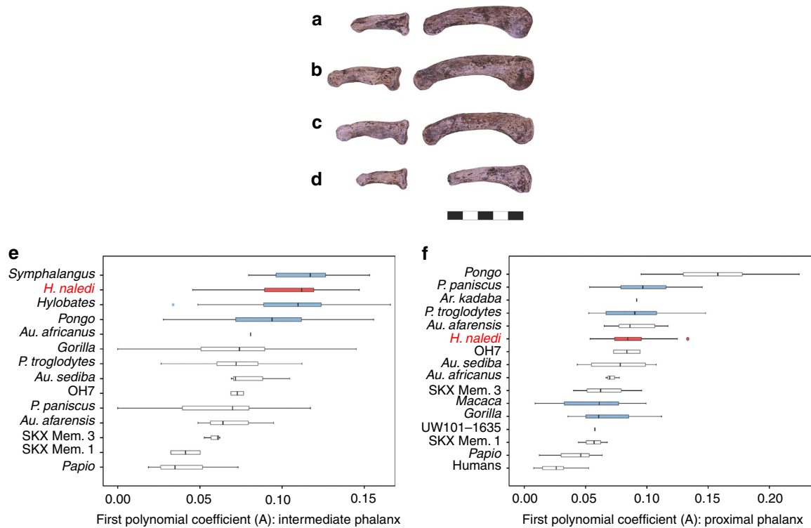
Figure 7 | Phalangeal curvature in H. naledi . Above, proximal and IPs of the Hand 1 ( a ) second, ( b ) third ( c ) fourth and ( d ) fifth ray in lateral view (all to scale). Below, box-and-whisker plots of curvature in H. naledi ( e ) intermediate phalanges ( n = 14 ) and ( f ) proximal phalanges ( n = 11 ), quantified as the first polynomial coefficient (A) of the polynomial functions ( y = Ax^2 + Bx + C ) representing longitudinal shaft curvature of the dorsal surface. Vertical line represents the median value, boxes show the interquartile range and whiskers extend to the highest and lowest values of each taxon, excluding outliers (dots). The H. naledi sample is shown in red and extant taxa that are not statistically distinct from this sample ( P \leq 0.05 based on one-way analysis of variance with Bonferroni correction) are shown in blue. 'SKX Mem. 1' and 'SKX Mem. 3' refer to the Swartkrans phalanx sample from Members 1 and 3, respectively, that can be attributed to either A. robustus or early Homo . 'UW 101-1635' is a juvenile H. naledi proximal phalanx. H. naledi is unusual compared with most other hominins in having both strongly curved proximal and intermediate phalanges.
