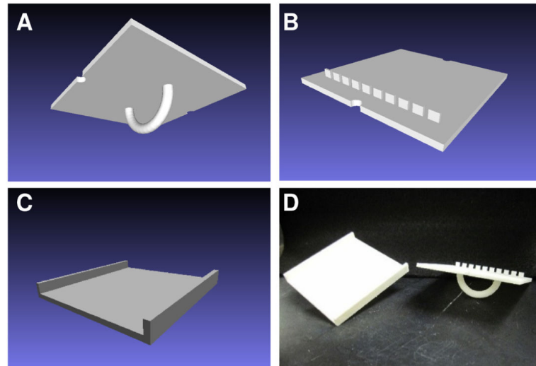
Figure 2. Methods for casting PAGE gels for use in horizontal electrophoresis setup A and B. 3D renderings of the top part of a casting mold for horizontal PAGE gels. C. 3D rendering of the bottom part of the casting mold. D. Digital photograph of the 3D printed casting mold for PAGE gels.
