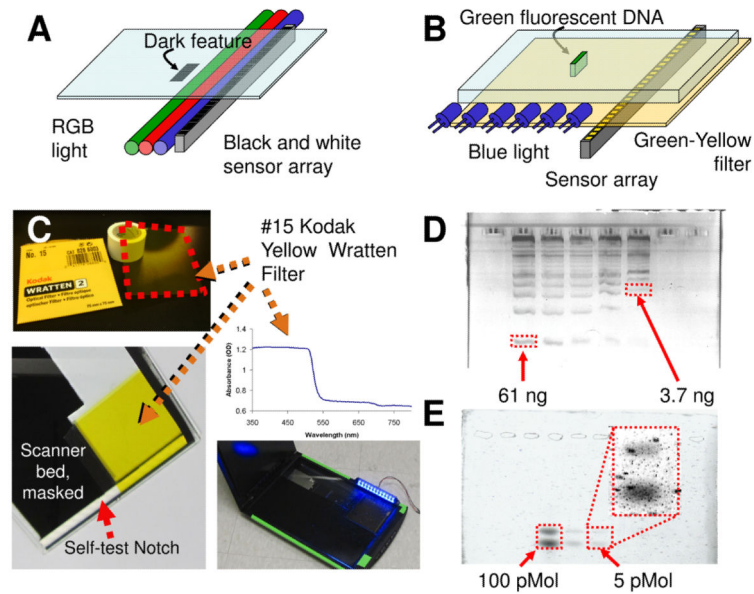
Figure 1. Design and performance of the converted gel scanner
