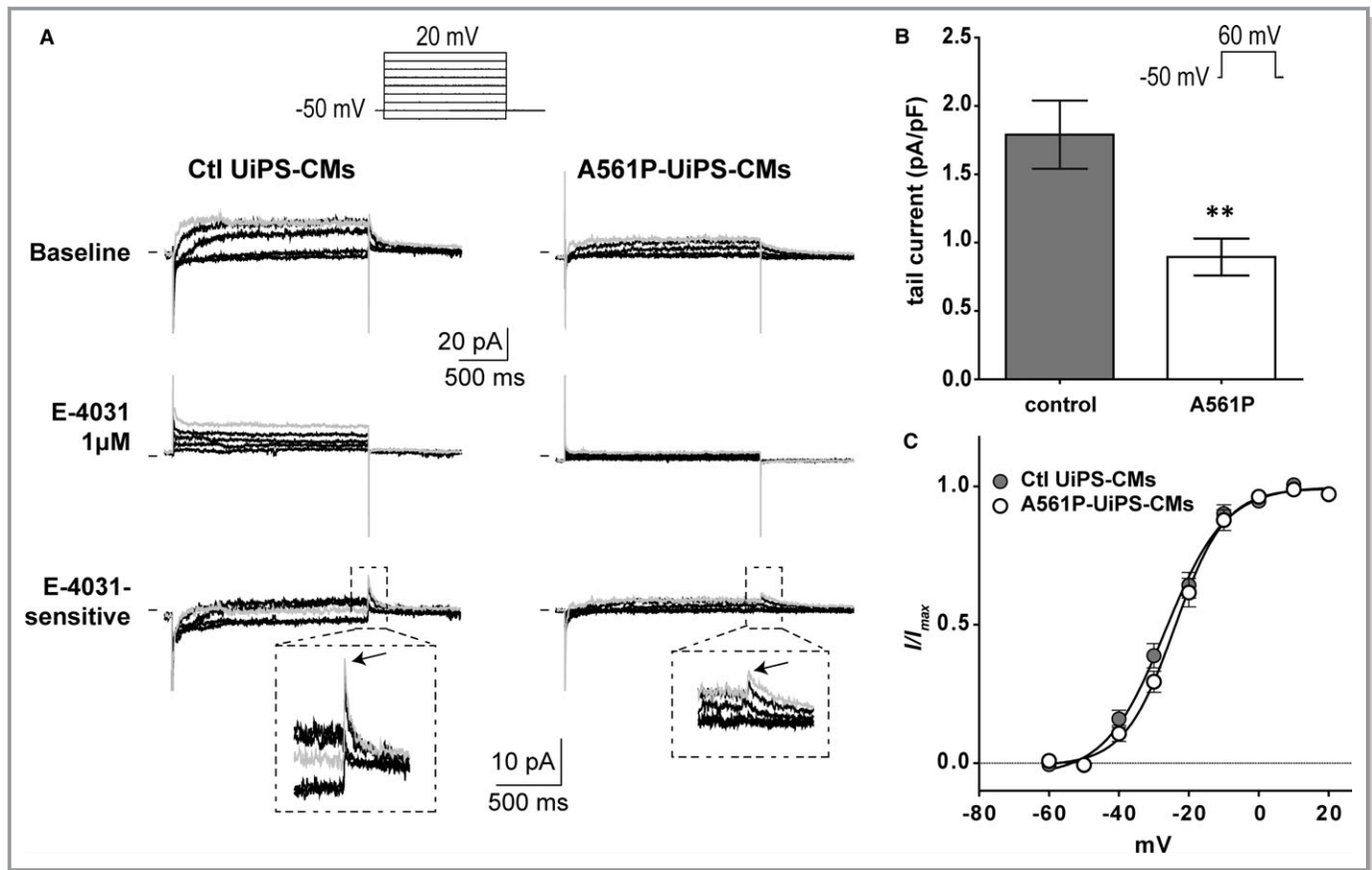
Figure 4. Reduction of delayed rectifier K + current ( I Kr ) density in A561P-UhiPS CMs. A, Representative raw data of currents recorded from control UhiPS-CMs (left) and A561P-UhiPS-CMs (right); protocol is shown as inset (holding potential: −50 mV; stimulation frequency: 1/12.5 Hz; traces with test pulse from −40 to 0 mV are shown). Currents are shown before and after 1 µmol/L E-4031 application. E-4031-sensitive currents are considered as I Kr . B, Tail current density measurement obtained on repolarization after test pulse at +60 mV in control UhiPS-CMs (n=13) and A561P-UhiPS CMs (n=11), highlighting a significant reduction in A561P-UhiPS CMs. Protocol is shown in inset. ** P <0.01 vs control UhiPS-CMs. C, Voltage-dependent activation curves obtained by plotting the relative E-4031-sensitive current on repolarization at −50 mV (arrows in A) in control UhiPS-CMs (n=13) and A561P-UhiPS CMs (n=8) (arrows in A). CM indicates cardiomyocytes; Ctrl, control; UhiPS, urine-derived human induced pluripotent stem cells.
