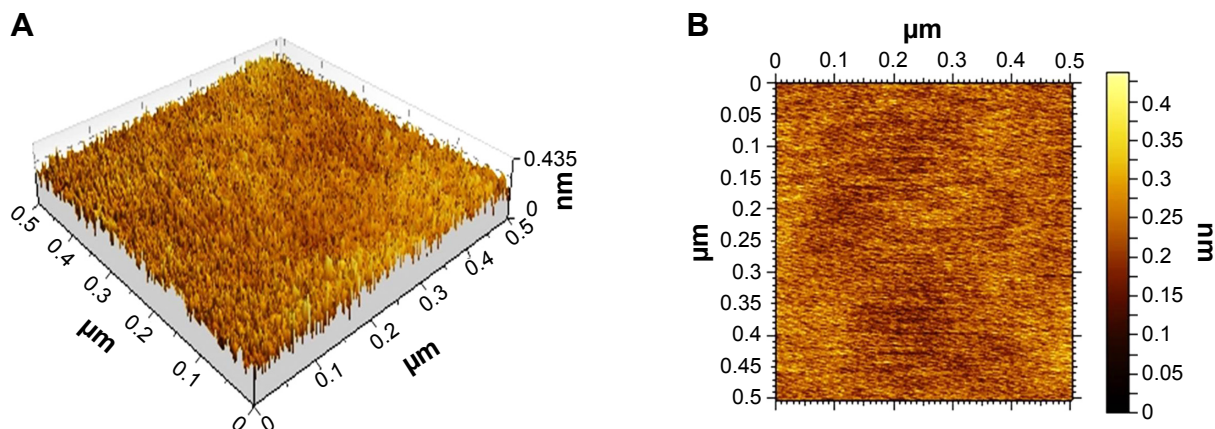
Figure 2 Surface topography of Zr_{48}Cu_{36}Al_8Ag_8 thin film metallic glass. Notes: (A) Three-dimensional view, (B) two-dimensional view.
