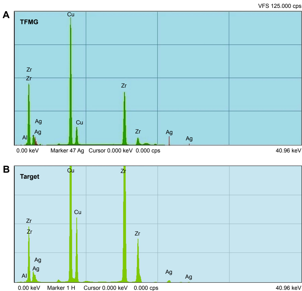
Figure 4 XRF spectra of the Zr-Cu-Al-Ag (A) thin film metallic glass and (B) target. Abbreviations: XRF, X-ray fluorescence; TFMG, thin film metallic glass.
