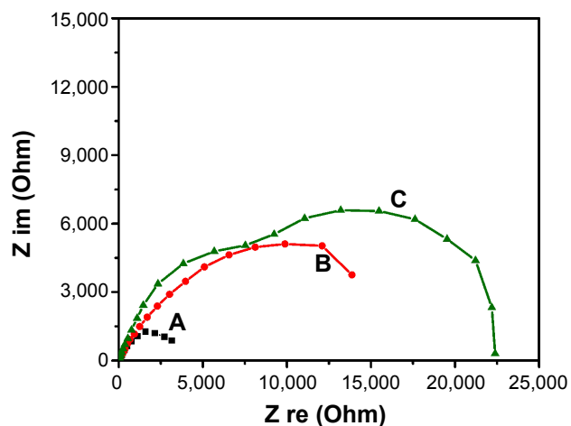
Figure 8 AC impedance studies of (A) blank stainless steel substrate, (B) 1.5 \mu m thick thin film metallic glass-coated stainless steel, and (C) 3 \mu m thick thin film metallic glass-coated stainless steel in simulated body fluid.
