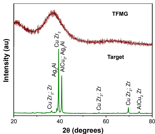
Figure 1 X-ray diffraction pattern of Zr_{48}Cu_{36}Al_8Ag_8 thin film metallic glass. Abbreviation: TFMG, thin film metallic glass.
