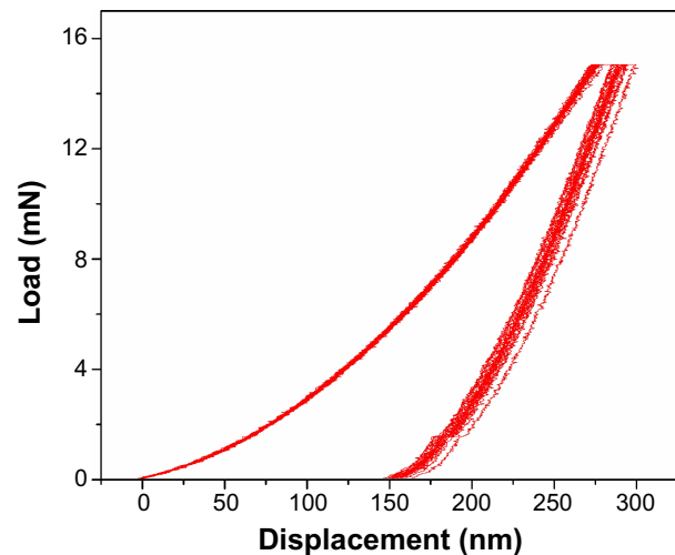
Figure 6 Load versus displacement nanoindentation curve obtained for Zr_{48}Cu_{36}Al_6Ag_8 thin film metallic glass.
