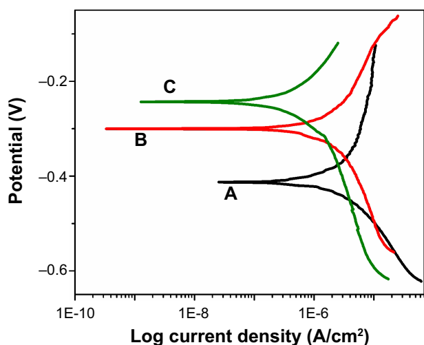
Figure 7 Tafel plots for (A) blank stainless steel substrate, (B) 1.5 \mu\text{m} thick thin film metallic glass-coated stainless steel, and (C) 3 \mu\text{m} thick thin film metallic glass-coated stainless steel in simulated body fluid.
