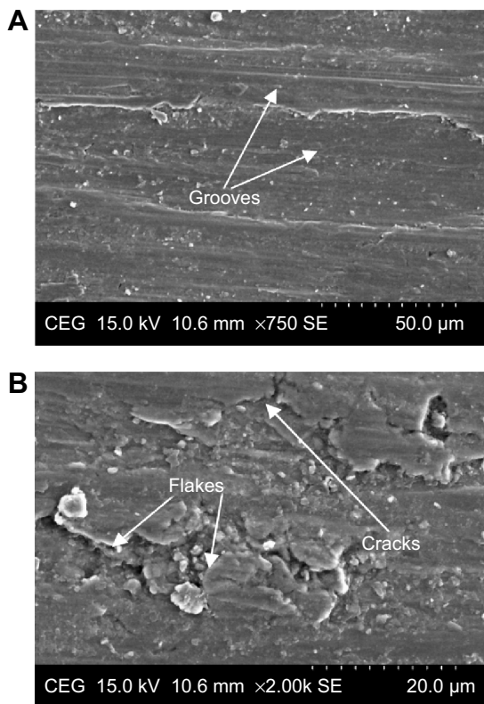
Figure 10 Scanning electron microscope image of wear track of the Ti-6Al-4V alloy. Notes: (A) Magnification 750×; (B) magnification 2,000×.
