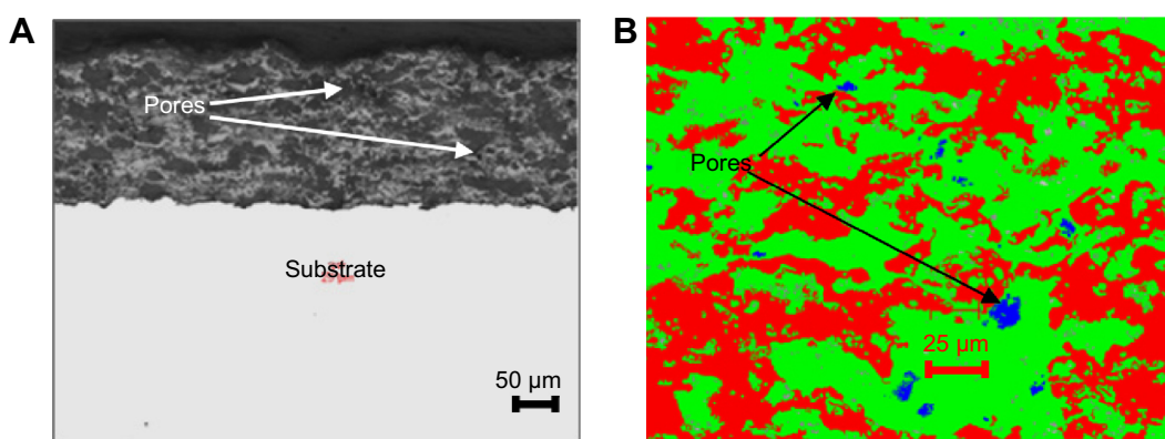
Figure 5 Optical micrographs of coating developed in optimal conditions. Notes: (A) Magnification 100 \times ; (B) magnification 200 \times .
