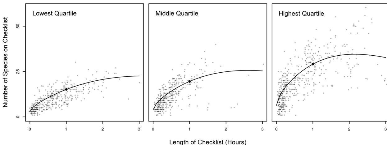
Fig 3. Representative Individual Species Accumulation Curves and Indices. Actual counts of species reported and observer-specific SACs for one individual observer classified as within the lowest quartile a), middle quartiles b), and highest quartile c). As the duration an observer spends collecting data for each checklist increases, the number of species observed increases. However as the duration lengthens, the rate of species accumulation decreases. The black dot on each curve is the SAC Index—the estimated number of species that individual would see during one hour of birding. Individuals were selected from the group who submitted at least 300 checklists between 2002 and 2012.
