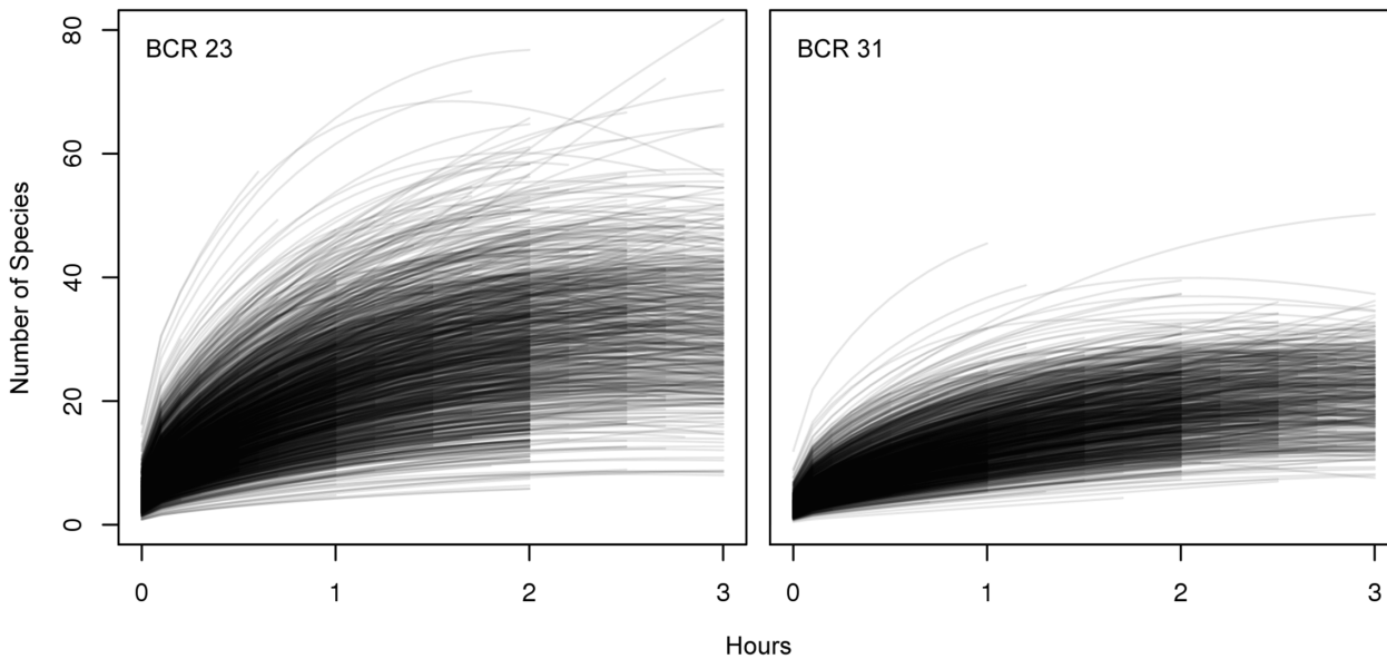
Fig 2. Species accumulation curves for all individual observers in a BCR. Each line represents the species accumulation curve derived from the mixed model fit to data from that BCR, for every individual observer in that BCR, and calculated with the standardized covariates of Sep 1 st , 7am start time, travelling 1km and average percentage land cover. The fitted line for each observer is plotted to the maximum count period duration in the data from that observer. Species accumulation curves that decrease for some observers may indicate different biases in attention to birding. For example checklists under 1 hour may be more concentrated birding, whereas checklists over 1 hour may combine birding with another activity such as hiking or fishing.
