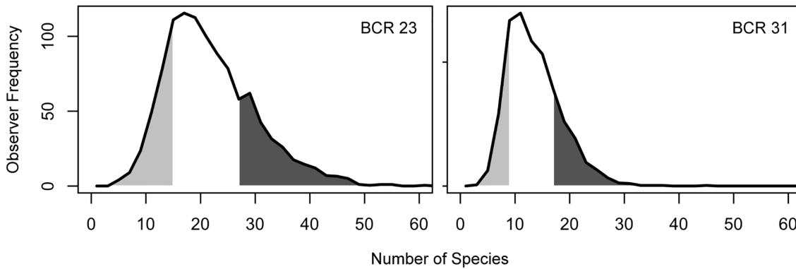
Fig 4. Distribution of individual SAC Indices. The expected number of species observed in 1 hour for all observers in a BCR. Individual data submission scores are ranked from lowest to highest and the light gray region represents the lower quartile of observers, and the dark gray region the upper quartile of observers.
