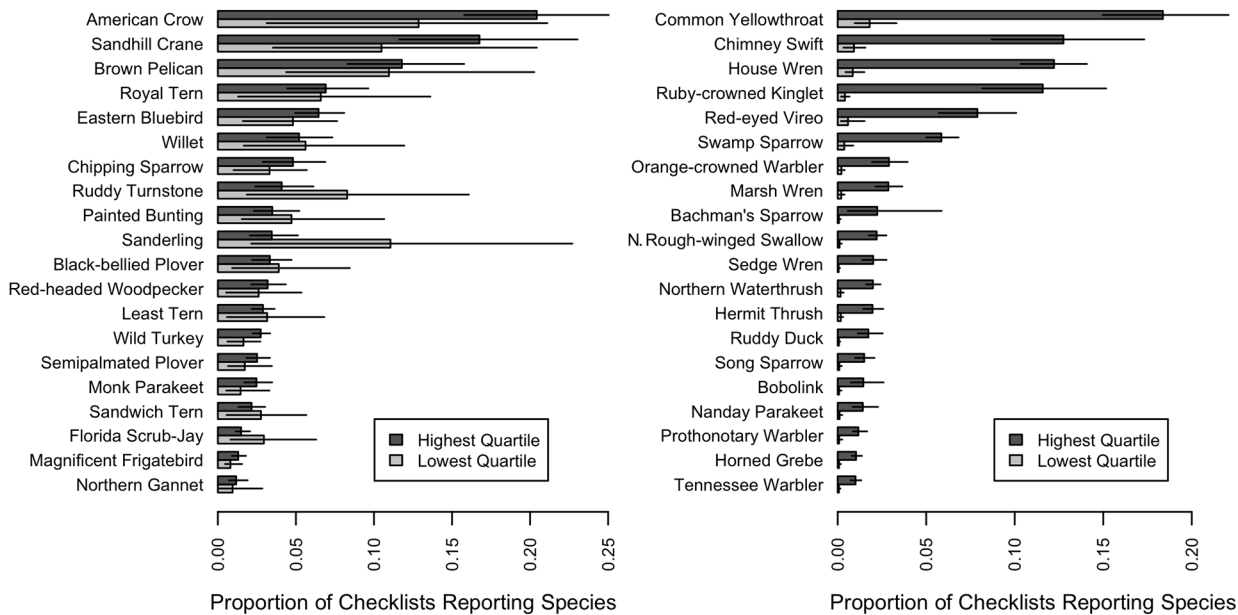
Fig 7. Bird species detected at the most similar and dis-similar rates by observers in the lowest quartile and highest quartile of SAC index values. Barplots from BCR 31 of the 20 species for which detection rates are proportionally most similar (left-hand panels) and the 20 species for which detection rates are proportionally most different (right-hand panels). Detection rate is the proportion of checklists that record a given species and error bars represent 95% bootstrap confidence intervals. The 20 species for which the two groups have proportionally most similar detection rates are generally species that are fairly easy to identify by sight. The 20 species that the two groups have proportionally most different detection rates are generally species that are difficult to identify, easier to identify by sound, or often be seen as a high-flying silhouette without many distinguishing features.
