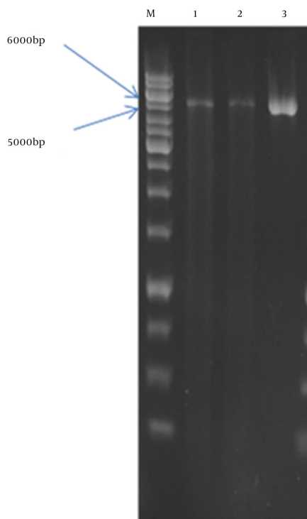
Figure 4. Analysis of Positive Clone With Restriction Enzyme XhoI
